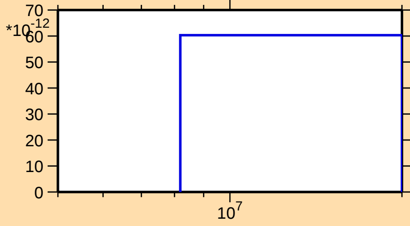
\sigma vs. E for ^{250}\text{Fm}(n,\text{He3})
