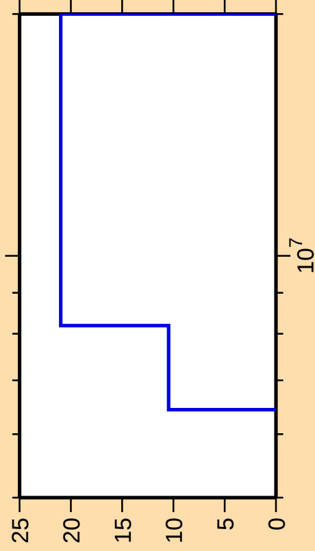
\Delta\sigma/\sigma vs. E for ^{250}\text{Fm}(n,d)
