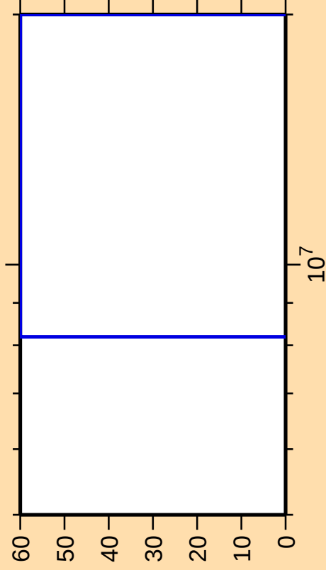
\Delta\sigma/\sigma vs. E for ^{250}\text{Fm}(n,\text{nd})
