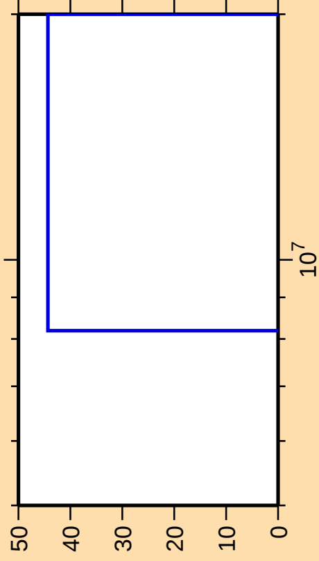
\Delta\sigma/\sigma vs. E for ^{250}\text{Fm}(n,p\alpha)
