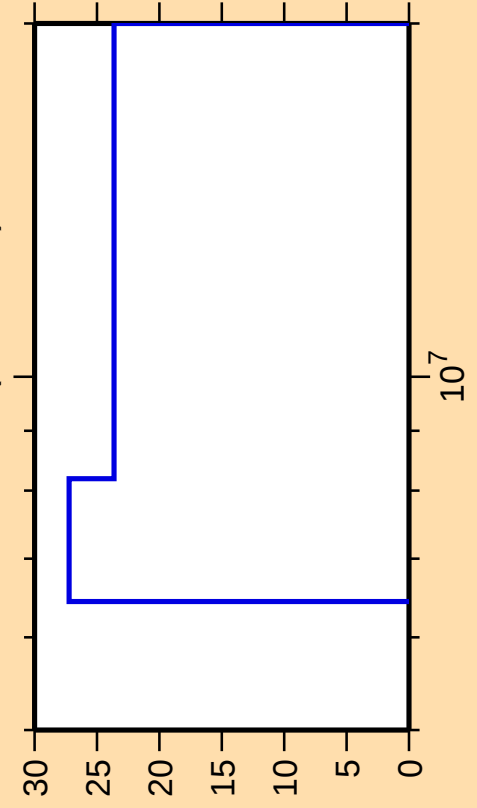
\Delta\sigma/\sigma vs. E for ^{250}\text{Fm}(n,n\text{cont.})
