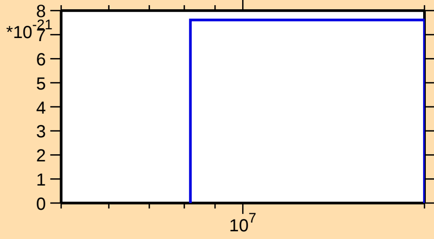
\sigma vs. E for ^{250}\text{Fm}(\text{mt } 42)
