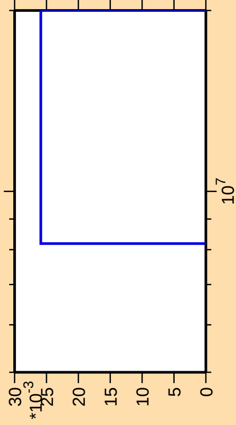
\Delta\sigma/\sigma vs. E for ^{250}\text{Fm}(\text{mt } 34)
