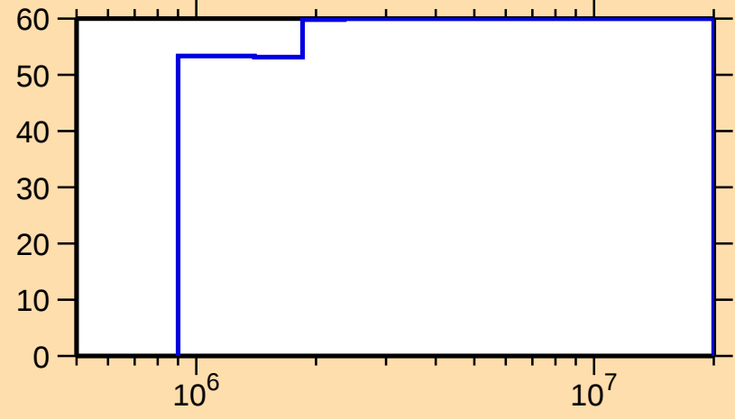
\Delta\sigma/\sigma vs. E for ^{250}\text{Fm}(n,n_1)
