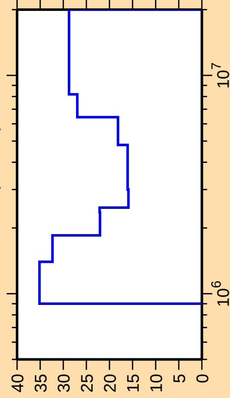
\Delta\sigma/\sigma vs. E for ^{250}\text{Fm}(n,\text{inel.})
