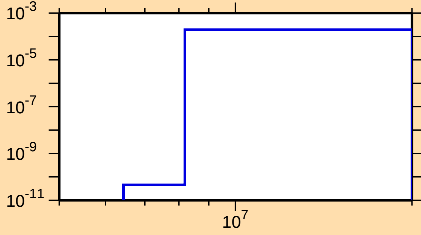
\sigma vs. E for ^{250}\text{Fm}(n,np)
