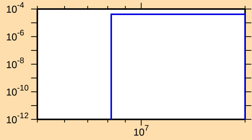
\sigma vs. E for ^{250}\text{Fm}(n,t)
