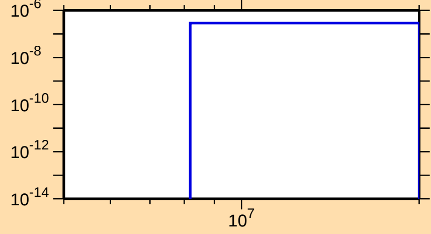
\sigma vs. E for ^{250}\text{Fm}(n,2n\alpha)
