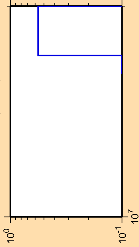
\Delta\sigma/\sigma vs. E for ^{250}\text{Fm}(\text{mt } 11)
