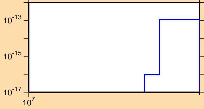
\sigma vs. E for ^{250}\text{Fm}(\text{mt } 11)
