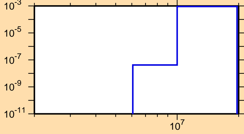
\sigma vs. E for ^{250}\text{Fm}(n,d)
