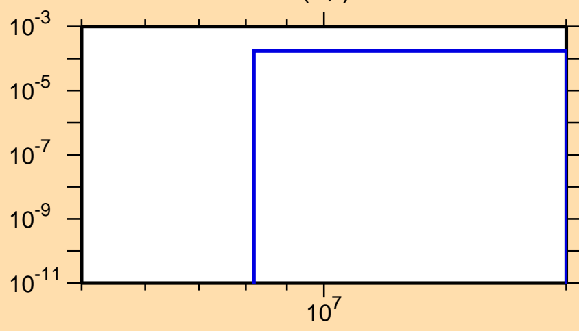
\sigma vs. E for ^{250}\text{Fm}(n,t)
