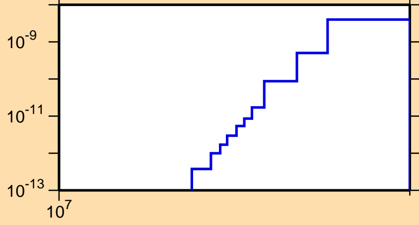
\sigma vs. E for ^{251}\text{Fm}(n,\text{He3})
