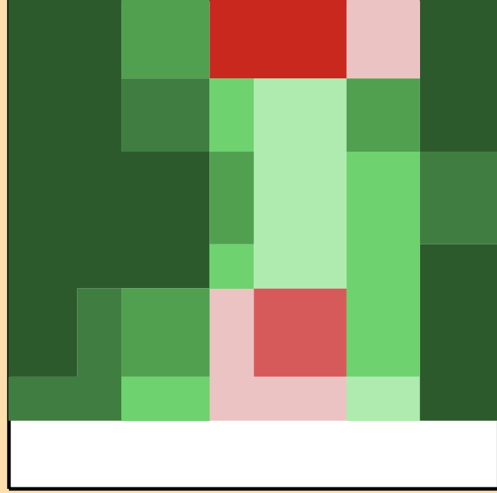
\Delta\sigma/\sigma vs. E for ^{251}\text{Fm}(n,\text{inel.})
