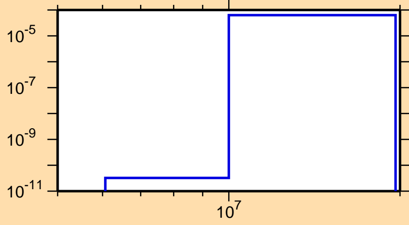
\sigma vs. E for ^{251}\text{Fm}(n,t)
