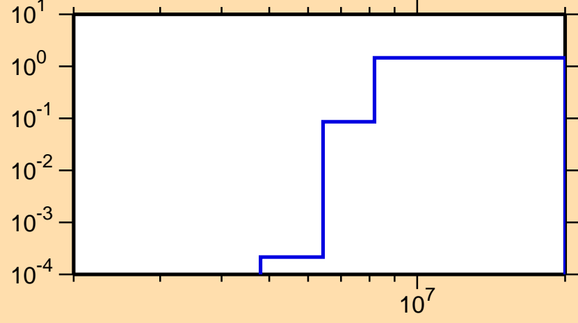
\sigma vs. E for ^{251}\text{Fm}(n,2n)
