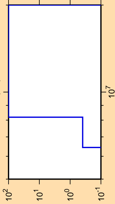
\Delta\sigma/\sigma vs. E for ^{251}\text{Fm}(n,t)
