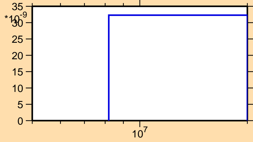
\sigma vs. E for ^{251}\text{Fm}(n,\text{nd})
