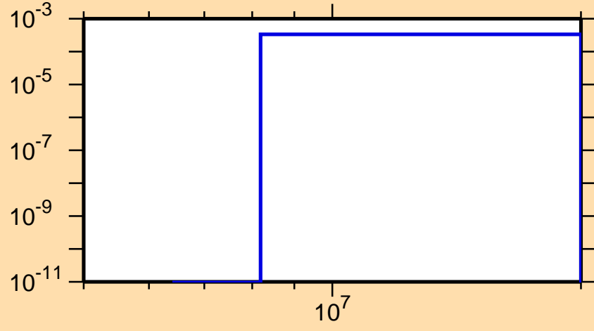
\sigma vs. E for ^{251}\text{Fm}(n,d)
