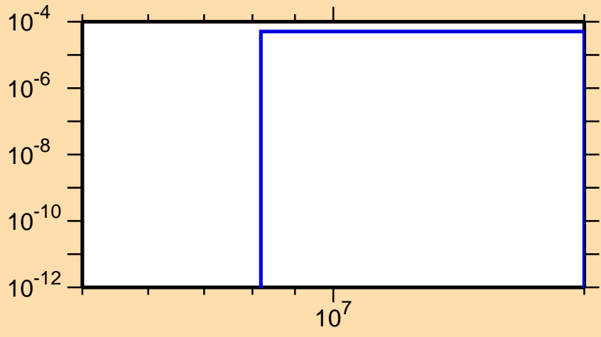
\sigma vs. E for ^{251}\text{Fm}(n,t)
