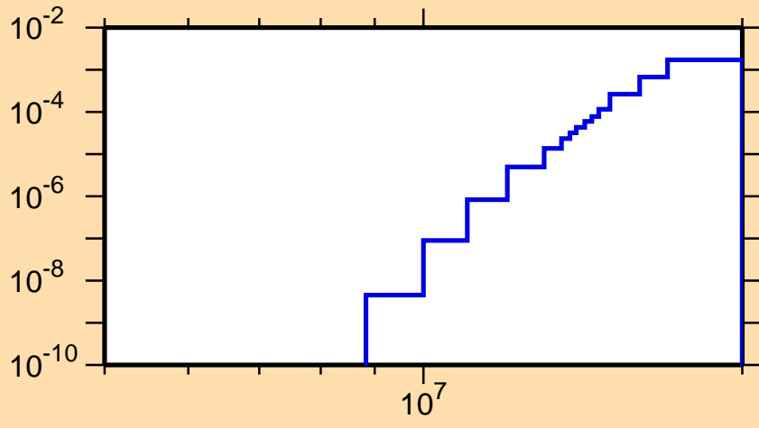
\sigma vs. E for ^{252}\text{Fm}(n,np)
