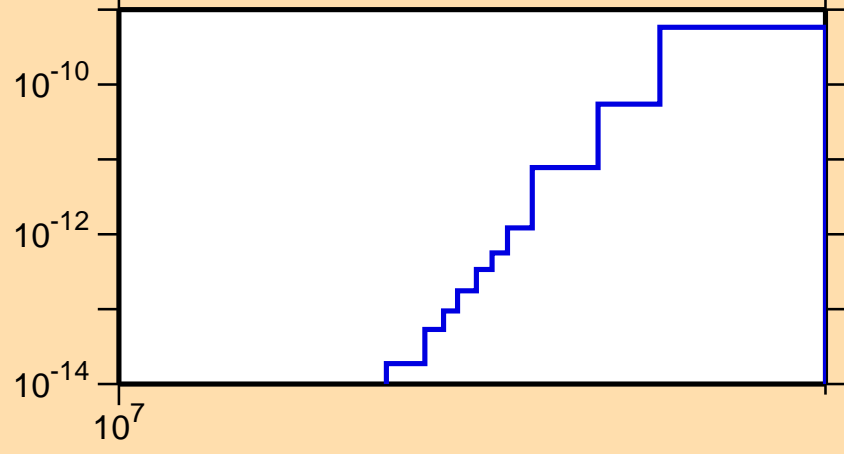
\sigma vs. E for ^{252}\text{Fm}(n,\text{He3})
