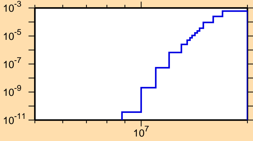
\sigma vs. E for ^{252}\text{Fm}(n,t)
