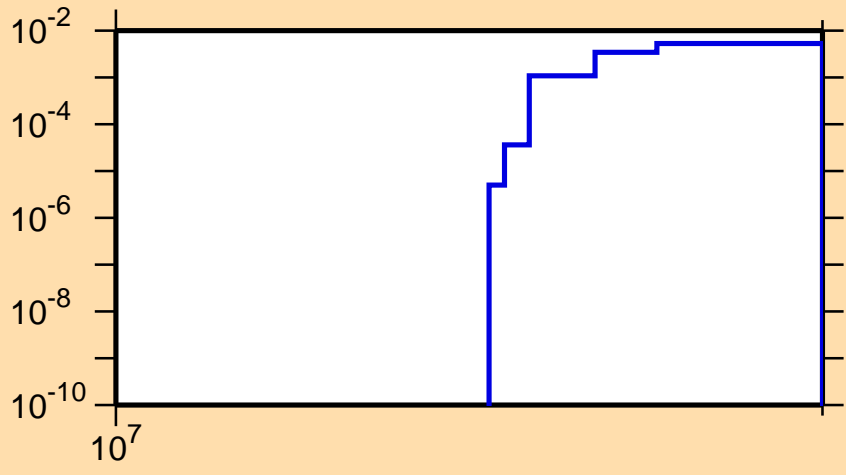
\sigma vs. E for ^{252}\text{Fm}(n,3n\alpha)
