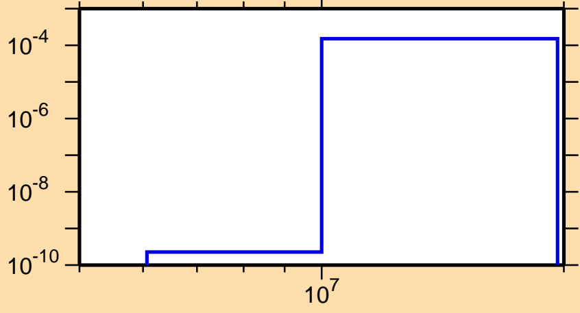
\sigma vs. E for ^{252}\text{Fm}(n,d)
