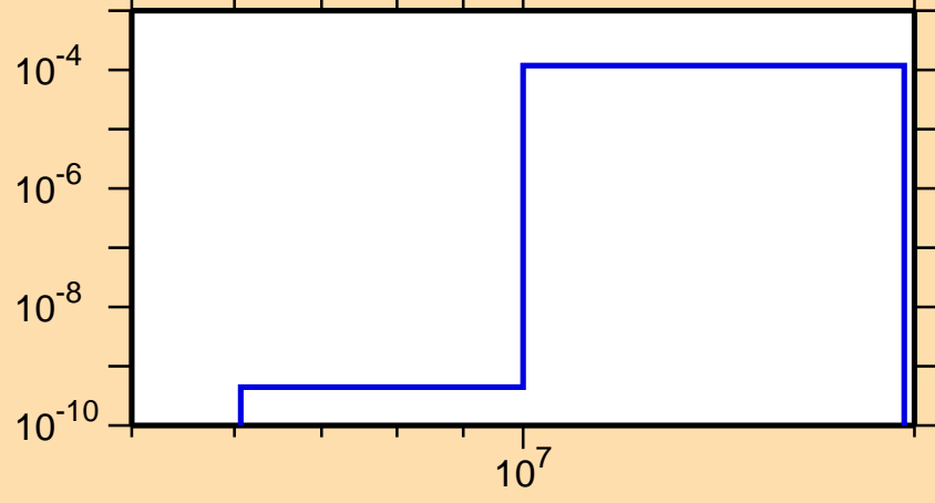
\sigma vs. E for ^{252}\text{Fm}(n,np)
