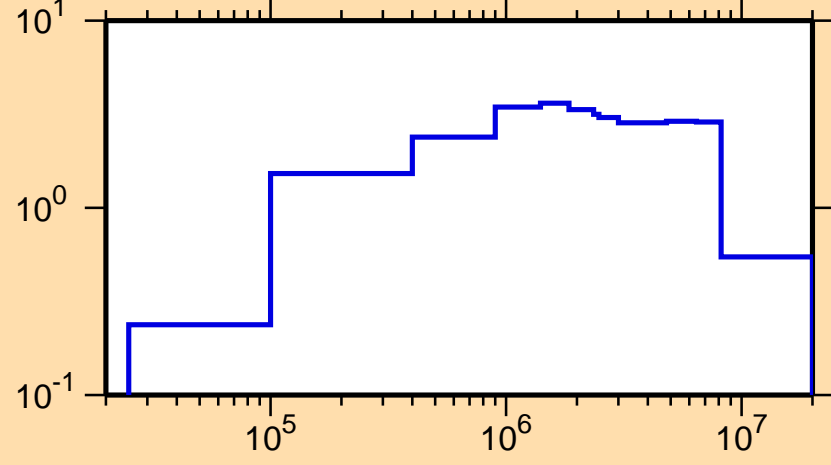
\sigma vs. E for ^{252}\text{Fm}(n,\text{inel.})
