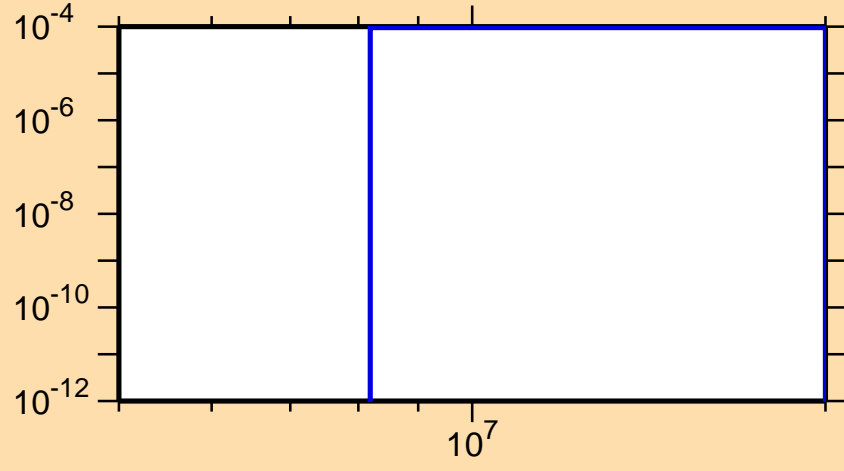
\sigma vs. E for ^{252}\text{Fm}(n,np)
