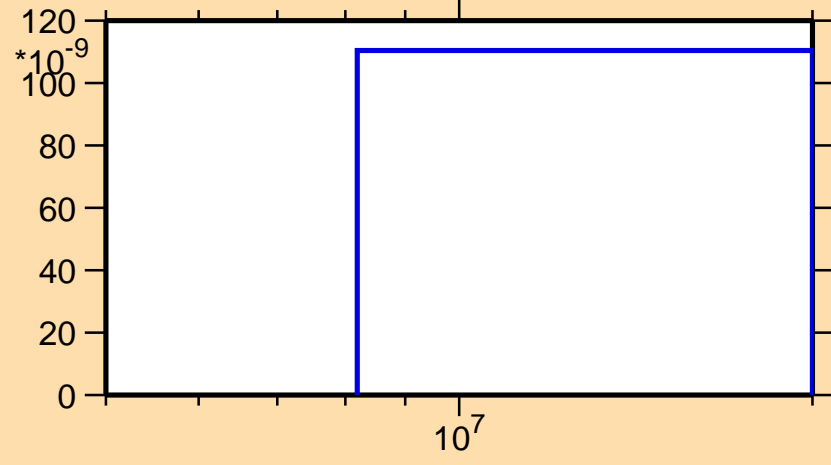
\sigma vs. E for ^{252}\text{Fm}(n,2n\alpha)
