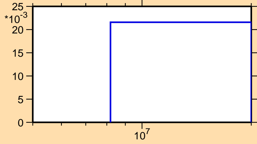
\sigma vs. E for ^{252}\text{Fm}(n,3n)
