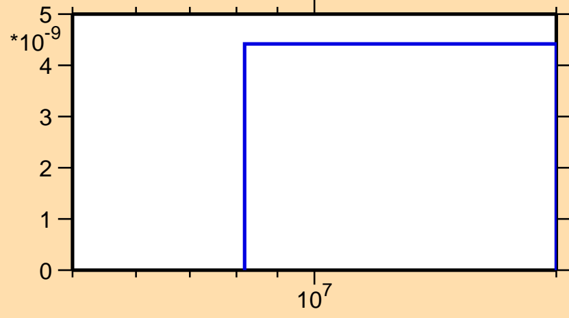
\sigma vs. E for ^{252}\text{Fm}(n,nd)
