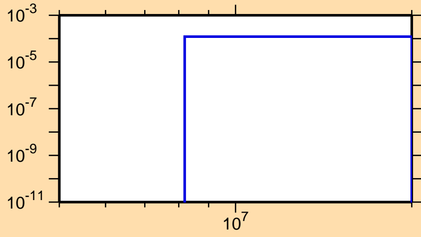
\sigma vs. E for ^{252}\text{Fm}(n,d)
