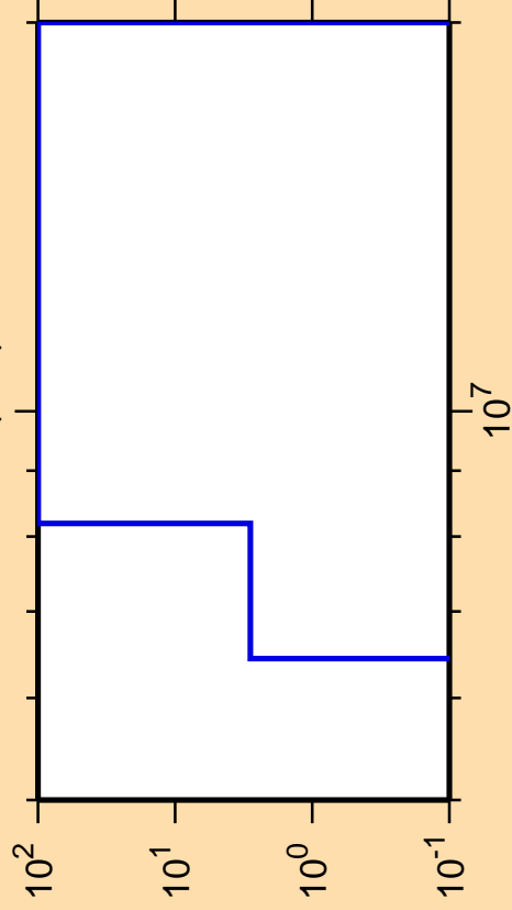
\Delta\sigma/\sigma vs. E for ^{252}\text{Fm}(n,d)
