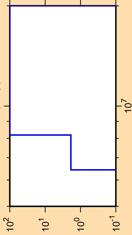
\Delta\sigma/\sigma vs. E for ^{252}\text{Fm}(n,np)
