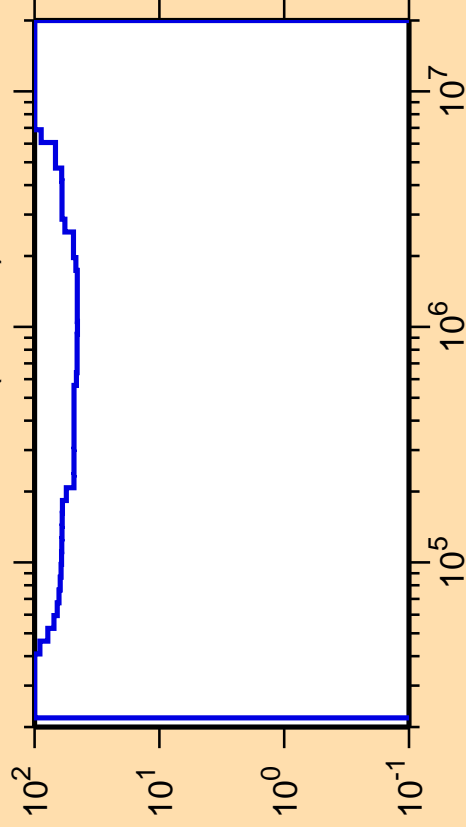
\Delta\sigma/\sigma vs. E for ^{253}\text{Fm}(n,\text{inel.})
