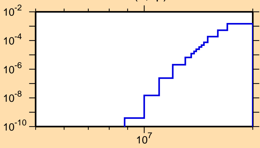
\sigma vs. E for ^{253}\text{Fm}(n,np)
