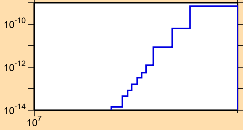
\sigma vs. E for ^{253}\text{Fm}(n,\text{He}3)
