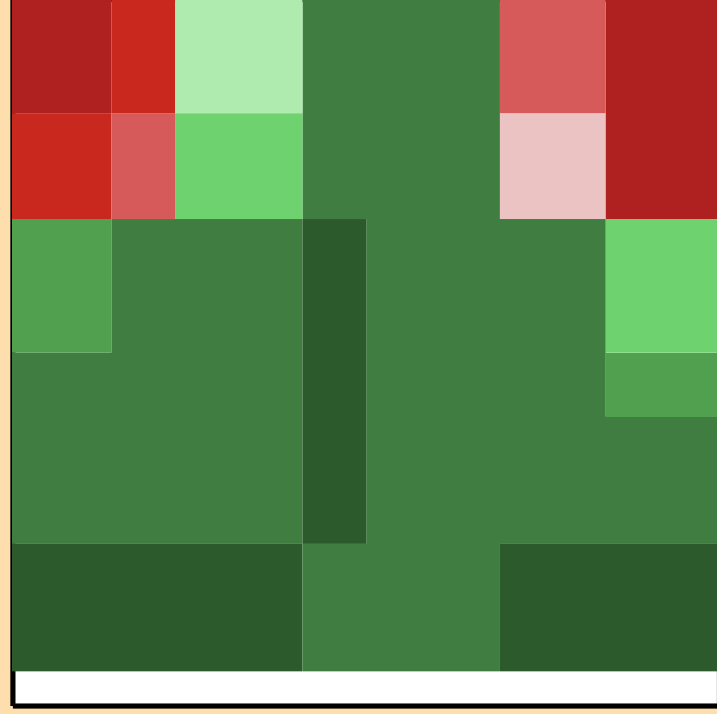
\Delta\sigma/\sigma vs. E for ^{253}\text{Fm}(n,\text{tot.})
