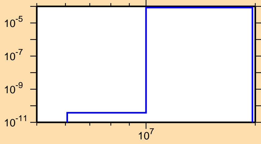
\sigma vs. E for ^{253}\text{Fm}(n,np)
