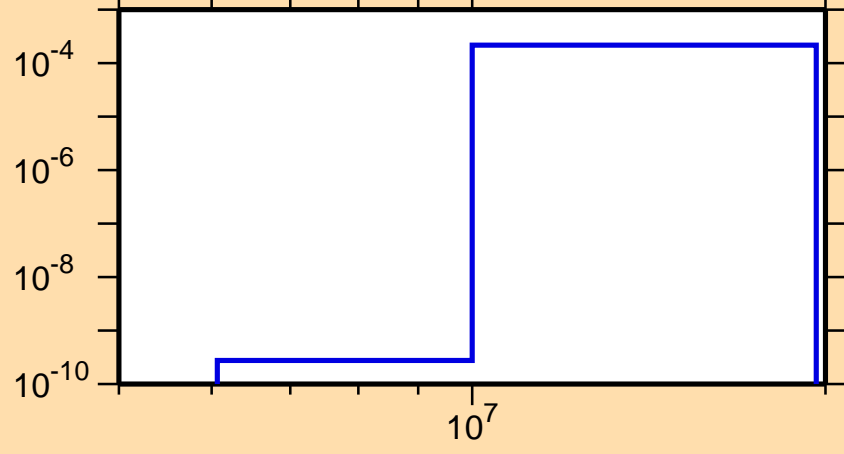
\sigma vs. E for ^{253}\text{Fm}(n,d)
