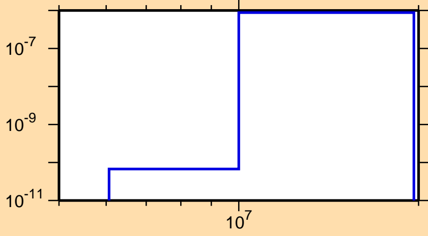
\sigma vs. E for ^{253}\text{Fm}(n,2n\alpha)
