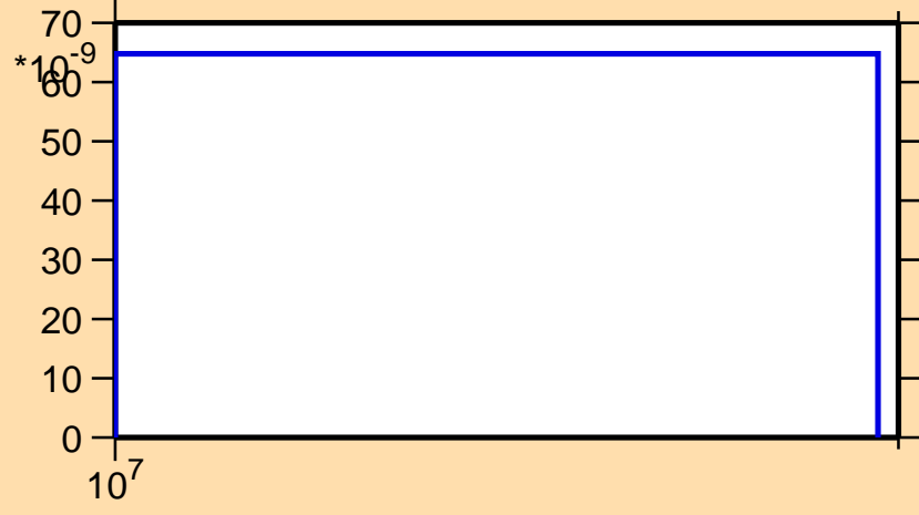
\sigma vs. E for ^{253}\text{Fm}(n,\text{nd})
