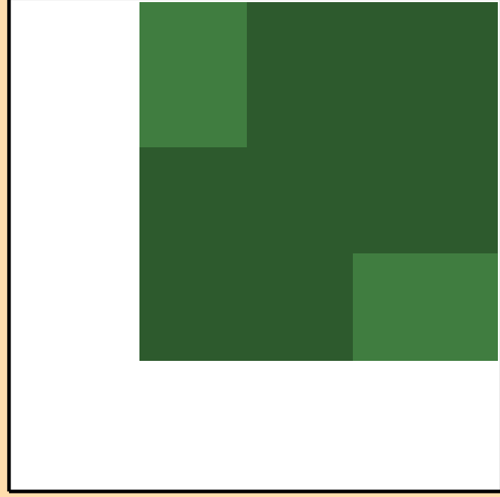
\sigma vs. E for ^{253}\text{Fm}(n,2n)
