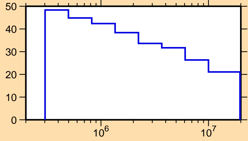
\Delta\sigma/\sigma vs. E for ^{253}\text{Fm}(n,n\text{onel.})
