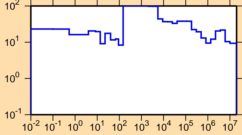
\Delta\sigma/\sigma vs. E for ^{253}\text{Fm}(n,\text{tot.})
