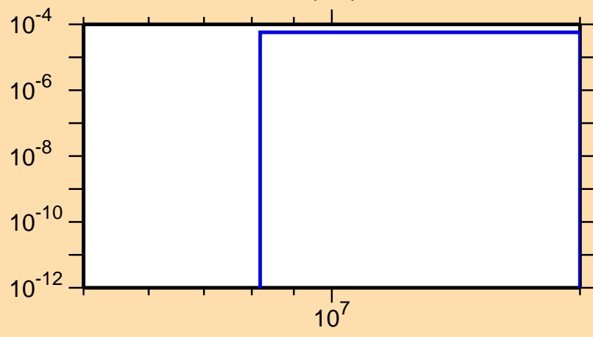
\sigma vs. E for ^{253}\text{Fm}(n,t)
