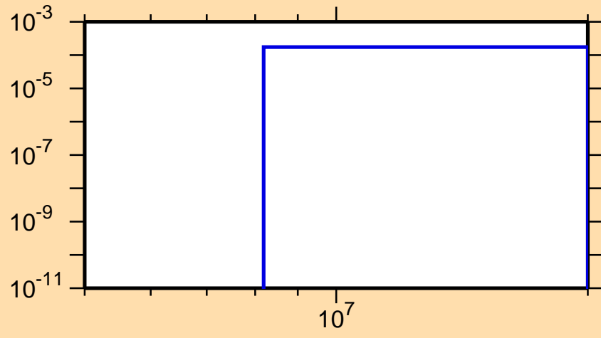
\sigma vs. E for ^{253}\text{Fm}(n,d)
