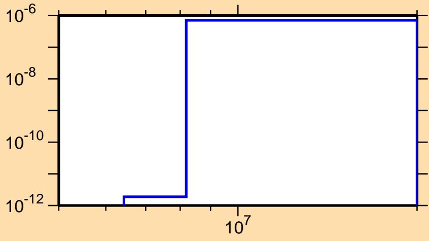
\sigma vs. E for ^{253}\text{Fm}(n,2n\alpha)
