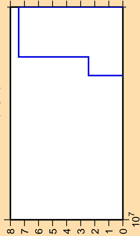
\Delta\sigma/\sigma vs. E for ^{254}\text{Fm}(n,p\alpha)
