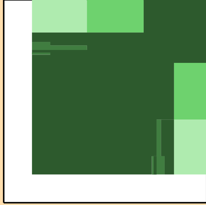
\sigma vs. E for ^{254}\text{Fm}(n,2n)
