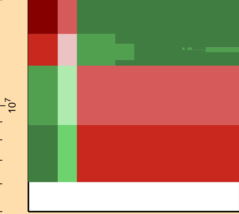
\Delta\sigma/\sigma vs. E for ^{254}\text{Fm}(n,\text{inel.})
