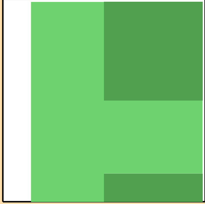
\Delta\sigma/\sigma vs. E for ^{254}\text{Fm}(n,2n)
