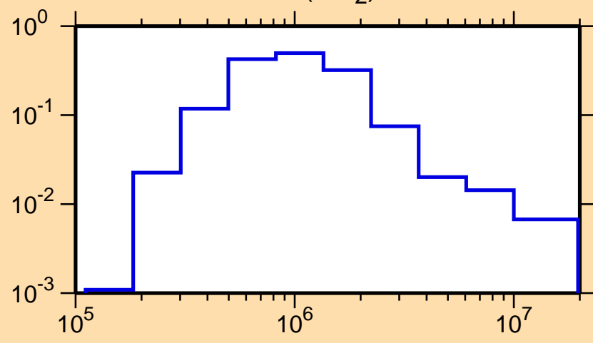
\sigma vs. E for ^{254}\text{Fm}(n,n_2)
