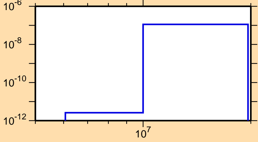
\sigma vs. E for ^{254}\text{Fm}(n,2n\alpha)
