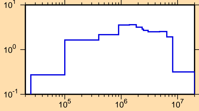
\sigma vs. E for ^{254}\text{Fm}(n,\text{inel.})
