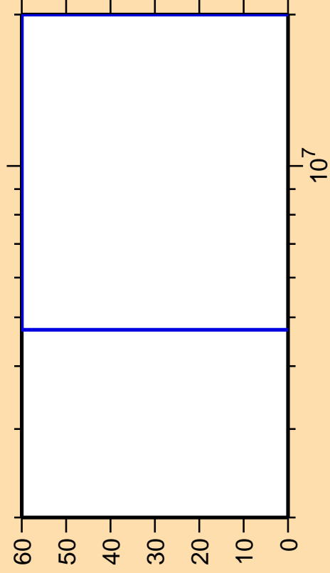
\Delta\sigma/\sigma vs. E for ^{255}\text{Fm}(n,\gamma)
