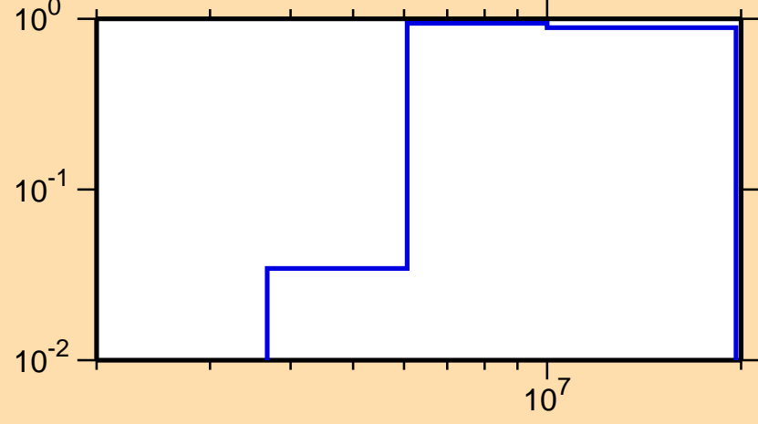
\sigma vs. E for ^{255}\text{Fm}(n,2n)
