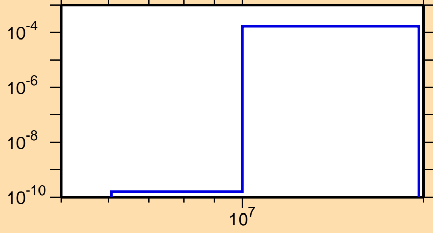
\sigma vs. E for ^{255}\text{Fm}(n,d)
