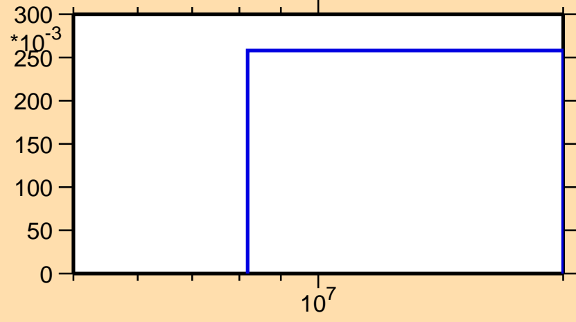
\sigma vs. E for ^{255}\text{Fm}(n,3n)
