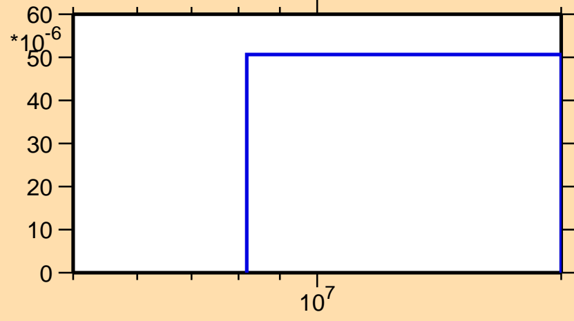
\sigma vs. E for ^{255}\text{Fm}(n,np)
