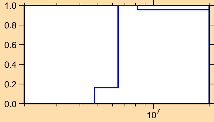
\sigma vs. E for ^{255}\text{Fm}(n,2n)
