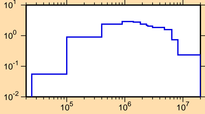
\sigma vs. E for ^{255}\text{Fm}(n,\text{inel.})
