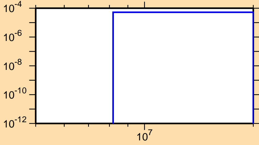
\sigma vs. E for ^{255}\text{Fm}(n,t)
