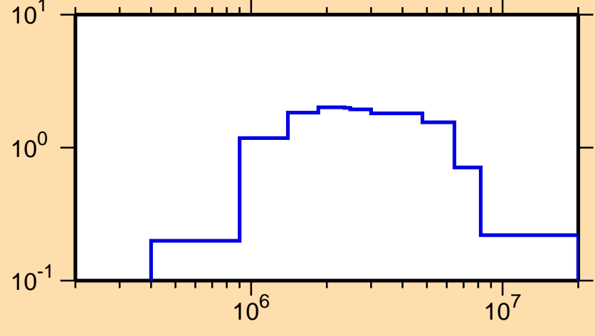
\sigma vs. E for ^{255}\text{Fm}(n,n\text{cont.})
