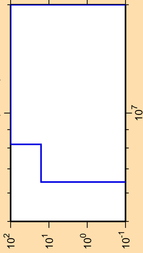
\Delta\sigma/\sigma vs. E for ^{255}\text{Fm}(n,2n\alpha)
