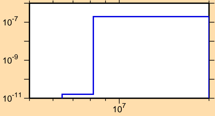
\sigma vs. E for ^{255}\text{Fm}(n,2n\alpha)
