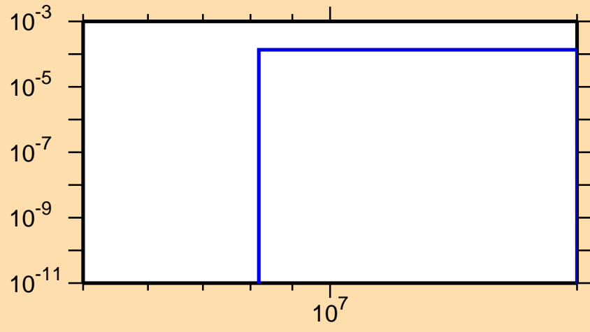
\sigma vs. E for ^{255}\text{Fm}(n,d)
