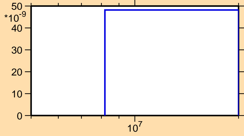
\sigma vs. E for ^{255}\text{Fm}(n,\text{nd})
