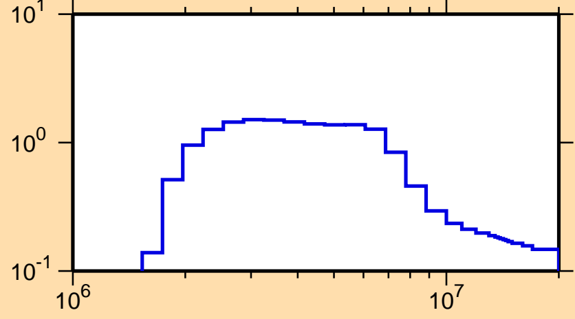
\sigma vs. E for ^{256}\text{Fm}(n,n\text{cont.})
