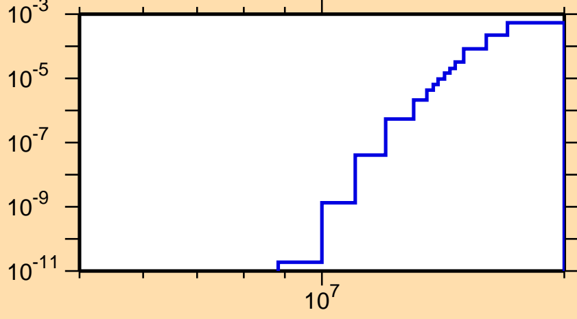
\sigma vs. E for ^{256}\text{Fm}(n,t)
