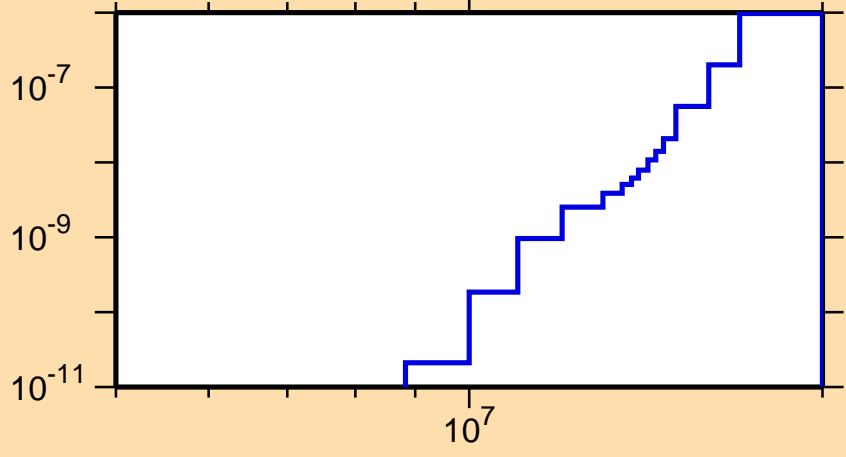
\sigma vs. E for ^{256}\text{Fm}(n,2n\alpha)
