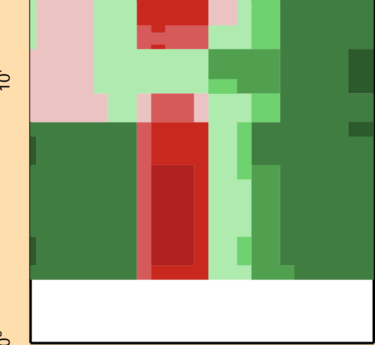
Correlation Matrix
