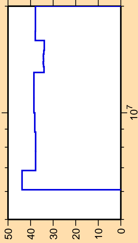
\Delta\sigma/\sigma vs. E for ^{256}\text{Fm}(n,f)
