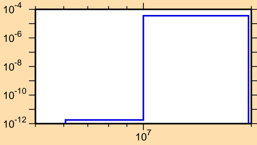
\sigma vs. E for ^{256}\text{Fm}(n,t)
