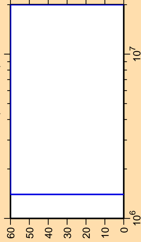
\Delta\sigma/\sigma vs. E for ^{256}\text{Fm}(n,ncont.)
