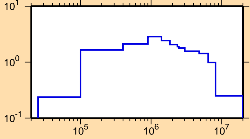
\sigma vs. E for ^{256}\text{Fm}(n,\text{inel.})
