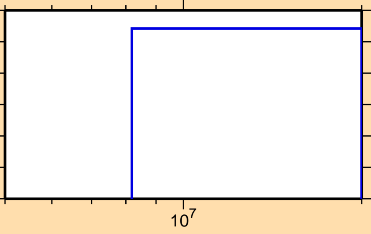
\sigma vs. E for ^{256}\text{Fm}(n,2n\alpha)
