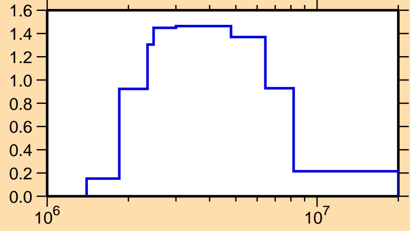
\sigma vs. E for ^{256}\text{Fm}(n,n\text{cont.})
