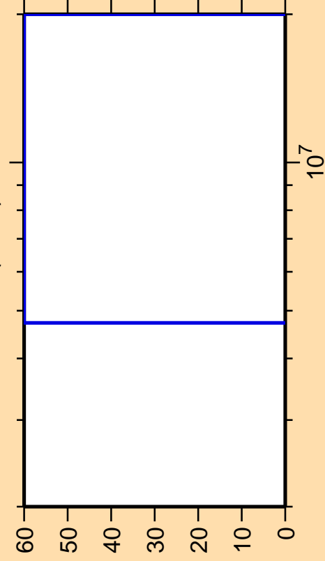
\Delta\sigma/\sigma vs. E for ^{257}\text{Fm}(n,2n)
