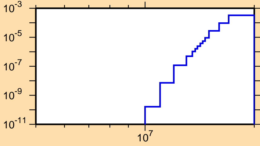
\sigma vs. E for ^{257}\text{Fm}(n,np)
