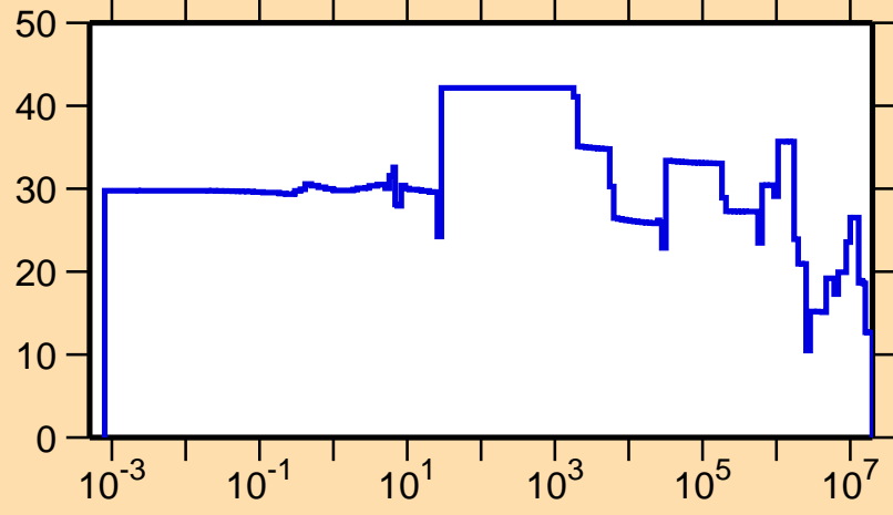
\Delta\sigma/\sigma vs. E for ^{257}\text{Fm}(n,\text{el.})
