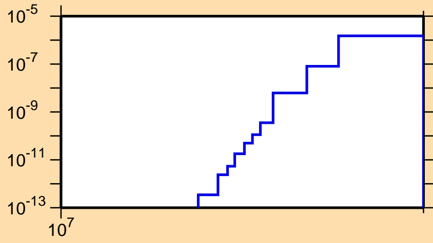
\sigma vs. E for ^{257}\text{Fm}(n,nd)
