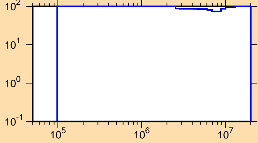
\Delta\sigma/\sigma vs. E for ^{257}\text{Fm}(n,\text{inel.})
