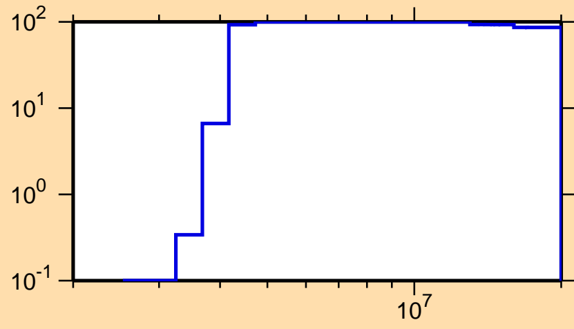
\Delta\sigma/\sigma vs. E for ^{257}\text{Fm}(n,p)
