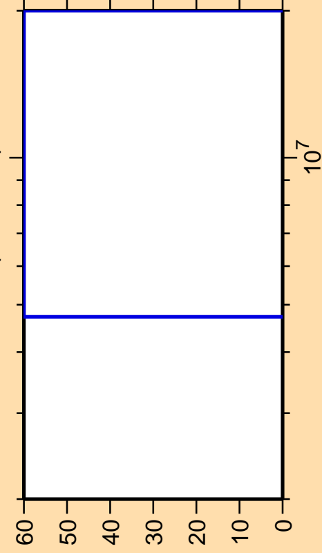
\Delta\sigma/\sigma vs. E for ^{257}\text{Fm}(n,n\text{cont.})
