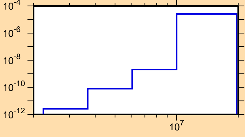
\sigma vs. E for ^{257}\text{Fm}(n,n\alpha)
