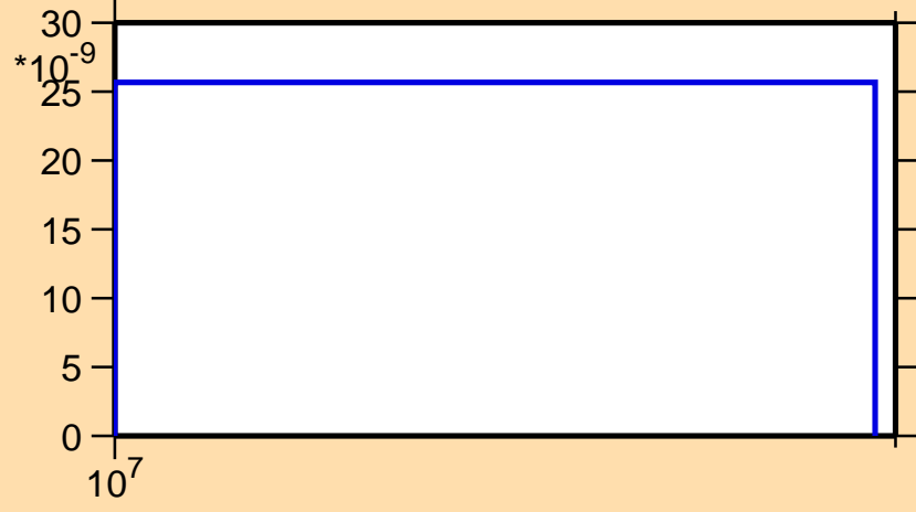
\sigma vs. E for ^{257}\text{Fm}(n,nt)
