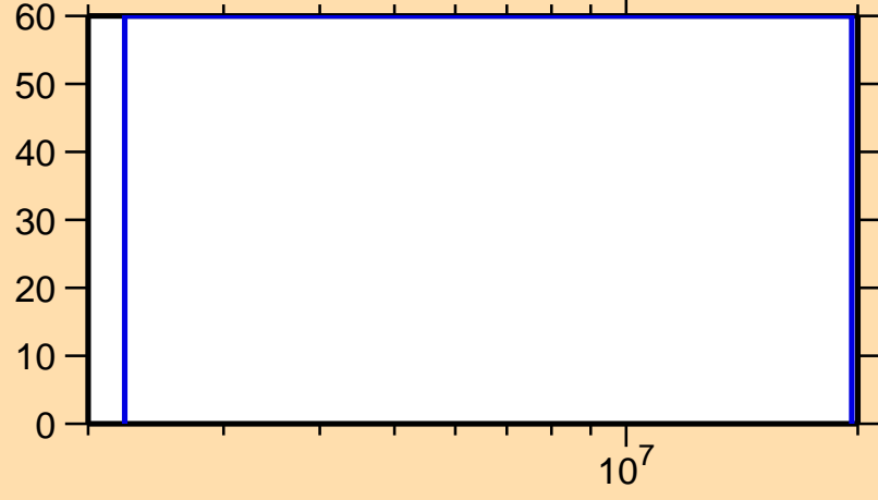
\Delta\sigma/\sigma vs. E for ^{257}\text{Fm}(n,ncont.)
