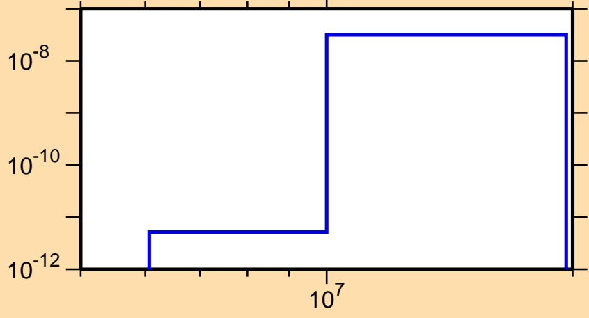
\sigma vs. E for ^{257}\text{Fm}(n,2n\alpha)
