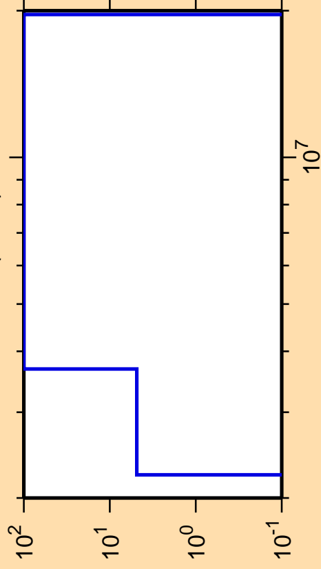
\Delta\sigma/\sigma vs. E for ^{257}\text{Fm}(n,n\alpha)
