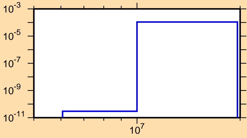
\sigma vs. E for ^{257}\text{Fm}(n,d)
