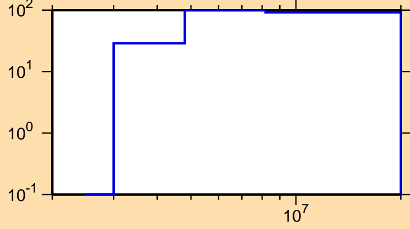
\Delta\sigma/\sigma vs. E for ^{257}\text{Fm}(n,p)
