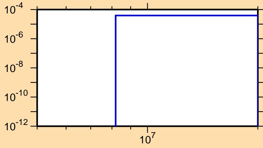
\sigma vs. E for ^{257}\text{Fm}(n,t)
