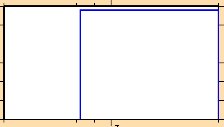
\sigma vs. E for ^{257}\text{Fm}(n,3n)
