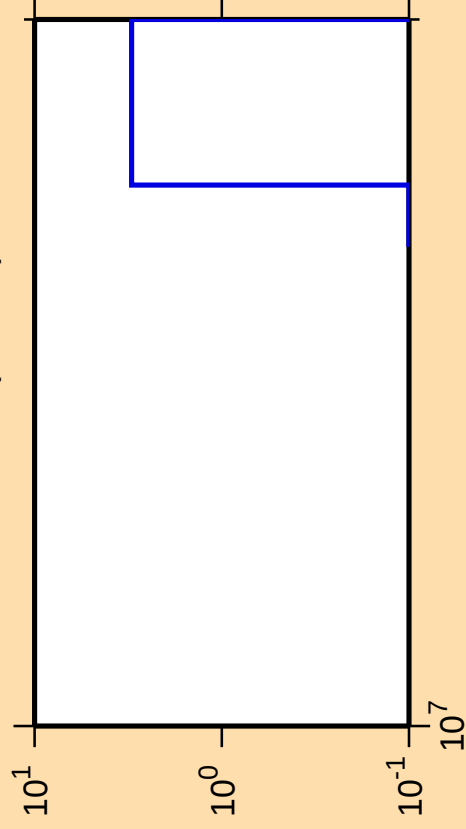
\Delta\sigma/\sigma vs. E for ^{259}\text{Fm}(n,\text{He3})
