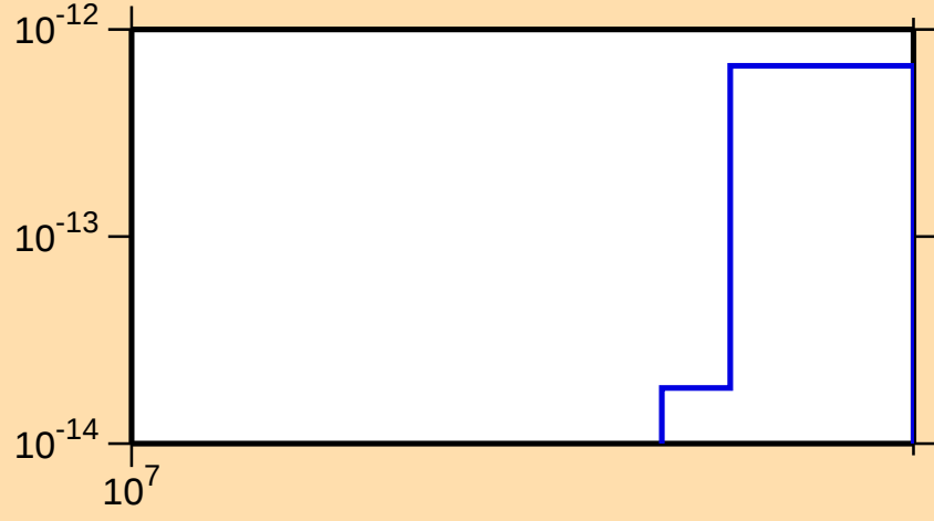
\sigma vs. E for ^{259}\text{Fm}(n,\text{He3})
