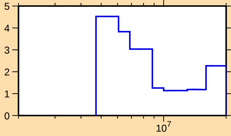
\Delta\sigma/\sigma vs. E for ^{259}\text{Fm}(n,\text{tot.})
