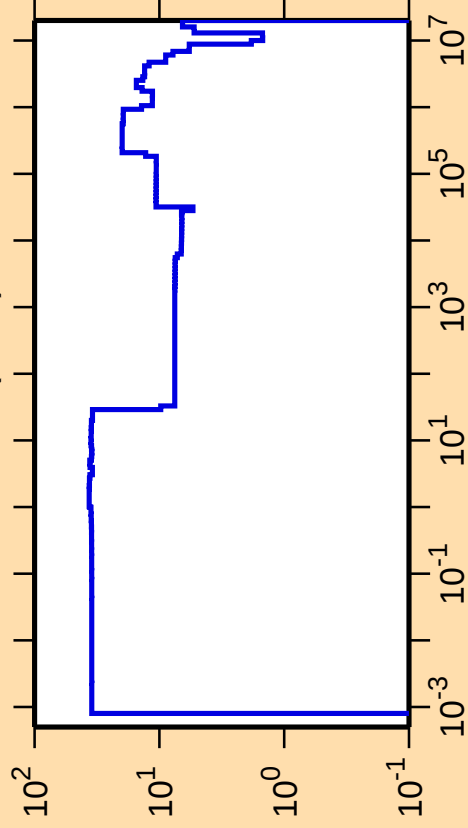
\Delta\sigma/\sigma vs. E for ^{259}\text{Fm}(n,\text{el.})
