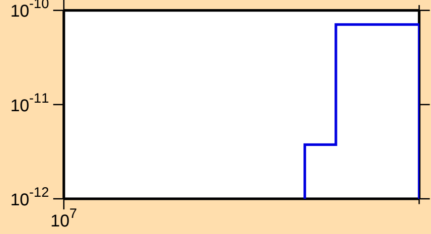
\sigma vs. E for ^{259}\text{Fm}(n,3n\alpha)
