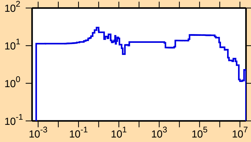
\Delta\sigma/\sigma vs. E for ^{259}\text{Fm}(n,\text{tot.})
