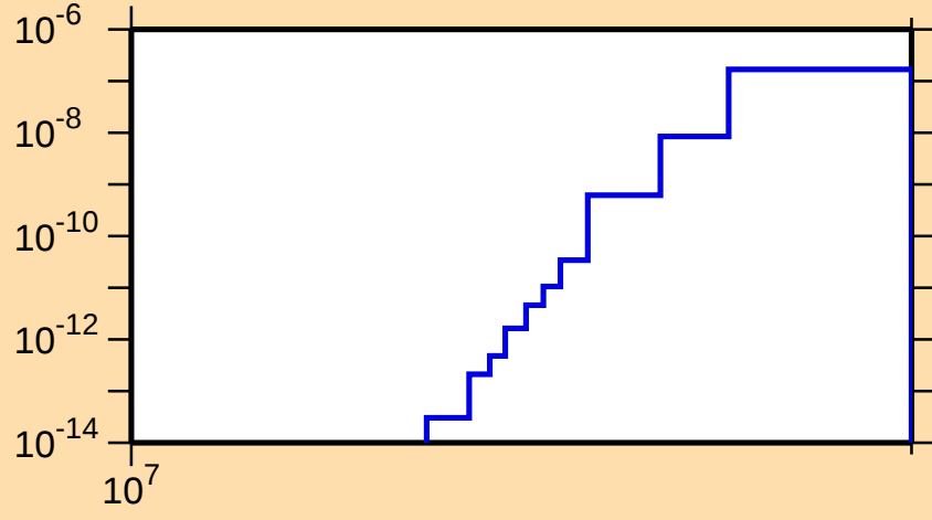
\sigma vs. E for ^{259}\text{Fm}(n,\text{nd})
