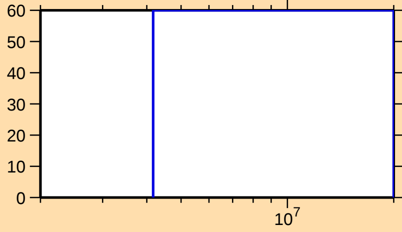
\Delta\sigma/\sigma vs. E for ^{259}\text{Fm}(n,\gamma)
