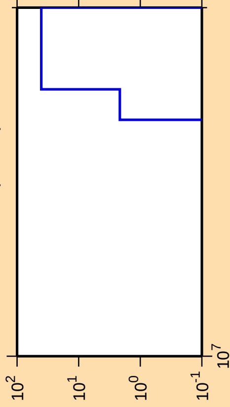
\Delta\sigma/\sigma vs. E for ^{259}\text{Fm}(n,3n\alpha)
