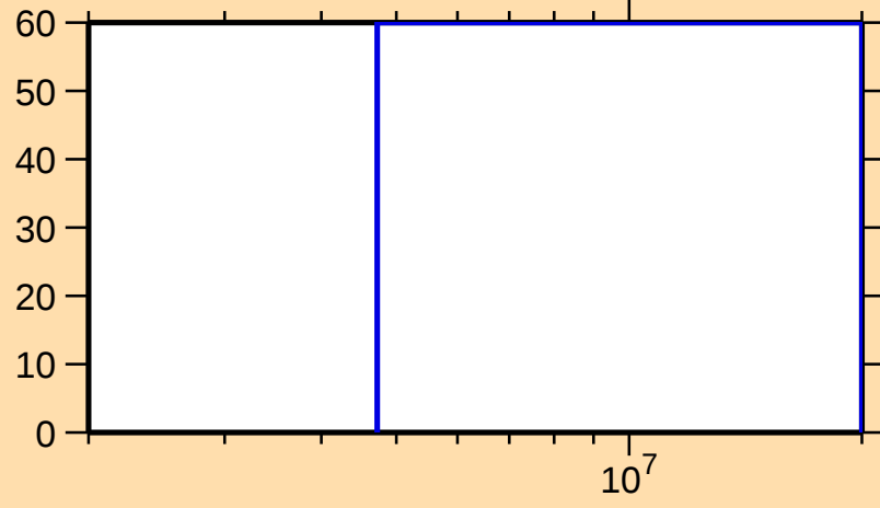
\Delta\sigma/\sigma vs. E for ^{259}\text{Fm}(n,2n)
