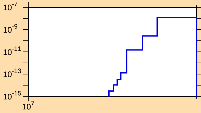
\sigma vs. E for ^{259}\text{Fm}(n,2np)
