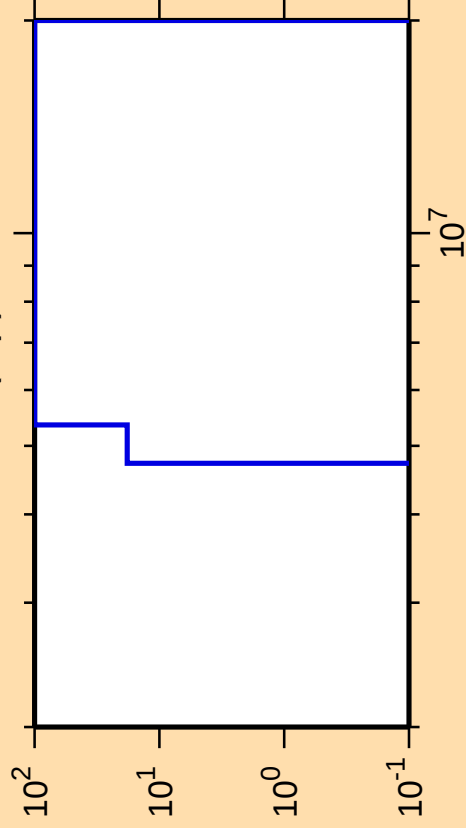
\Delta\sigma/\sigma vs. E for ^{259}\text{Fm}(n,p)
