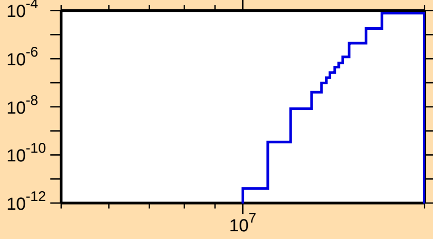
\sigma vs. E for ^{259}\text{Fm}(n,np)
