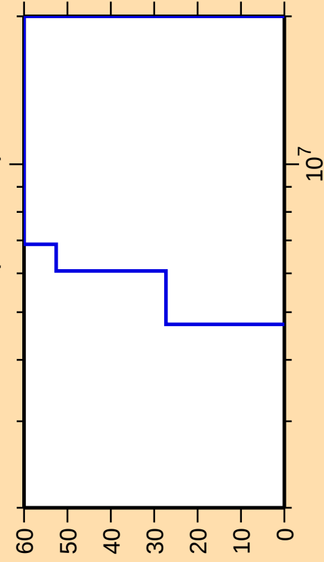
\Delta\sigma/\sigma vs. E for ^{259}\text{Fm}(n,n\text{cont.})
