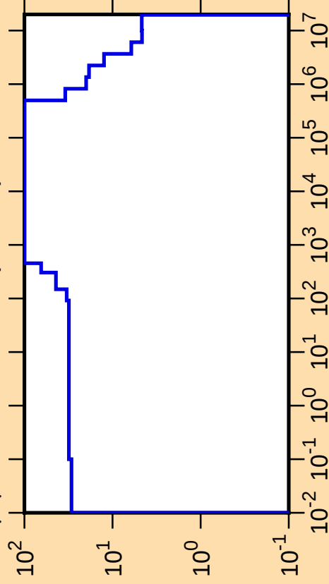
\Delta\mu/\mu vs. E for ^{259}\text{Fm}(\text{mt251})
