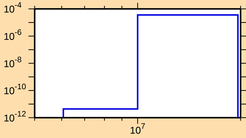
\sigma vs. E for ^{259}\text{Fm}(n,t)
