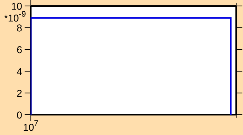
\sigma vs. E for ^{259}\text{Fm}(n,nt)
