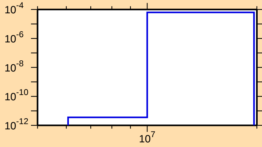
\sigma vs. E for ^{259}\text{Fm}(n,d)
