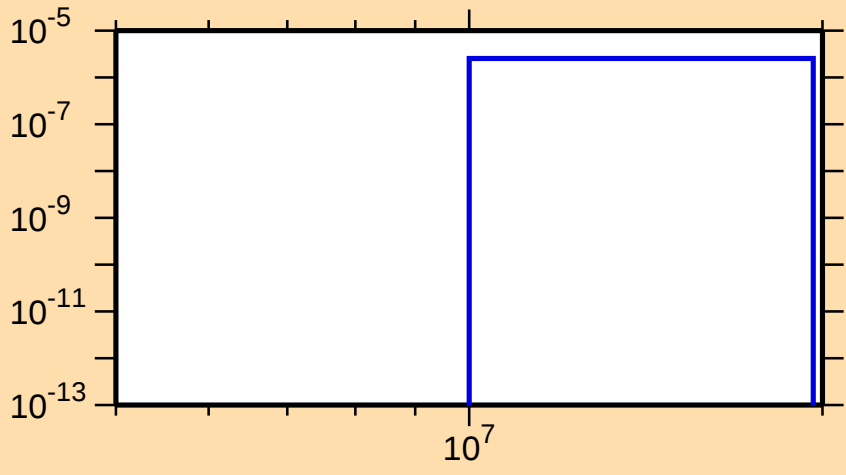
\sigma vs. E for ^{259}\text{Fm}(n,np)
