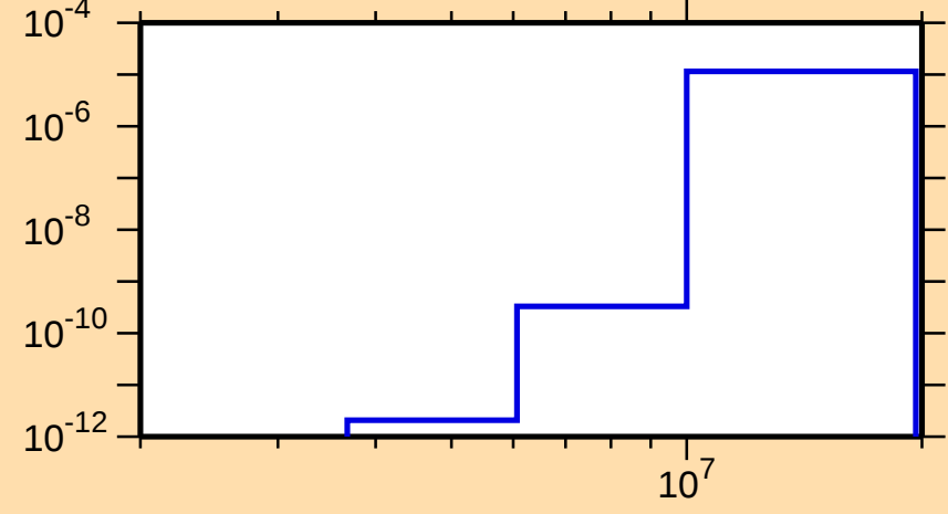
\sigma vs. E for ^{259}\text{Fm}(n,n\alpha)
