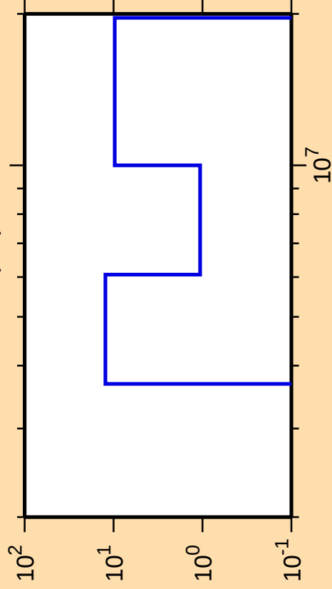
\Delta\sigma/\sigma vs. E for ^{259}\text{Fm}(n,f)
