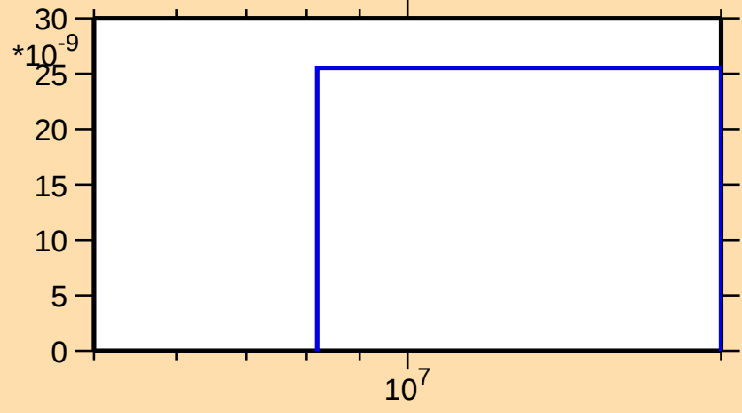
\sigma vs. E for ^{259}\text{Fm}(n,2n\alpha)
