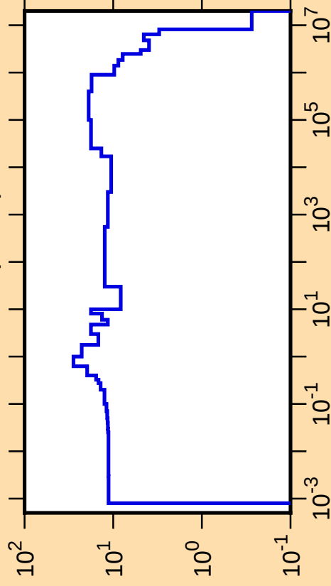
\Delta\sigma/\sigma vs. E for ^{259}\text{Fm}(n,\text{tot.})
