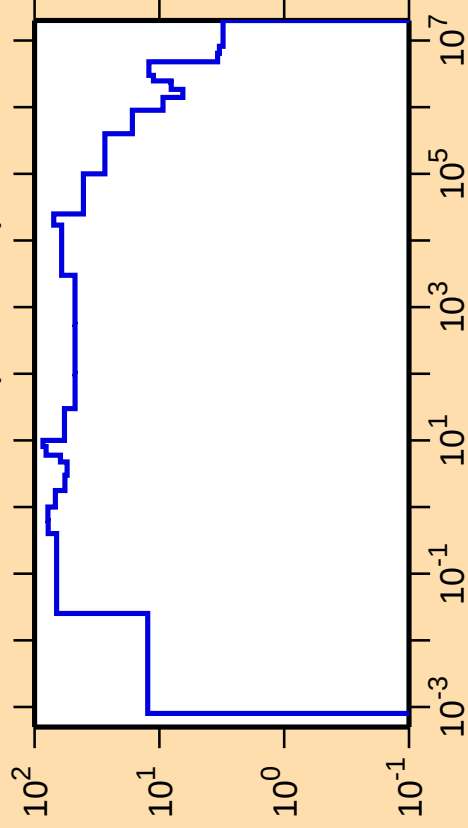
\Delta\sigma/\sigma vs. E for ^{259}\text{Fm}(n,\text{nonel.})
