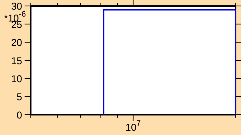
\sigma vs. E for ^{259}\text{Fm}(n,t)
