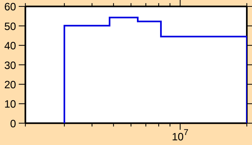
\Delta\sigma/\sigma vs. E for ^{259}\text{Fm}(n,n_1)
