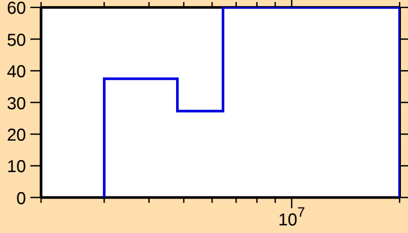
\Delta\sigma/\sigma vs. E for ^{259}\text{Fm}(n,n\text{cont.})
