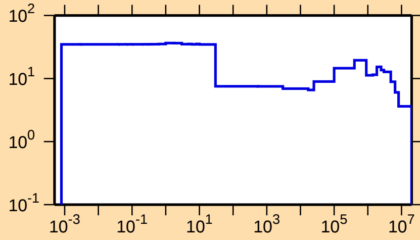
\Delta\sigma/\sigma vs. E for ^{259}\text{Fm}(n,\text{el.})
