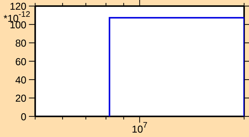
\sigma vs. E for ^{259}\text{Fm}(n,2np)
