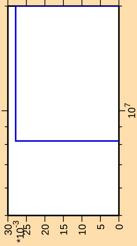
\Delta\sigma/\sigma vs. E for ^{259}\text{Fm}(n,\text{He3})
