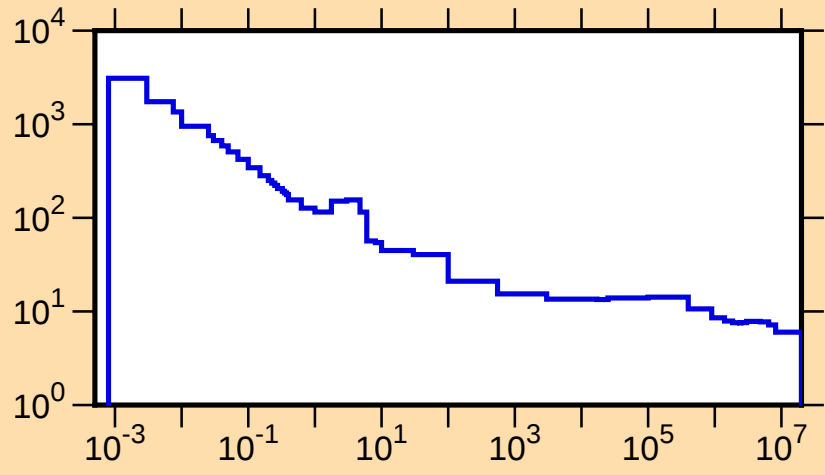
\sigma vs. E for ^{259}\text{Fm}(n,\text{tot.})
