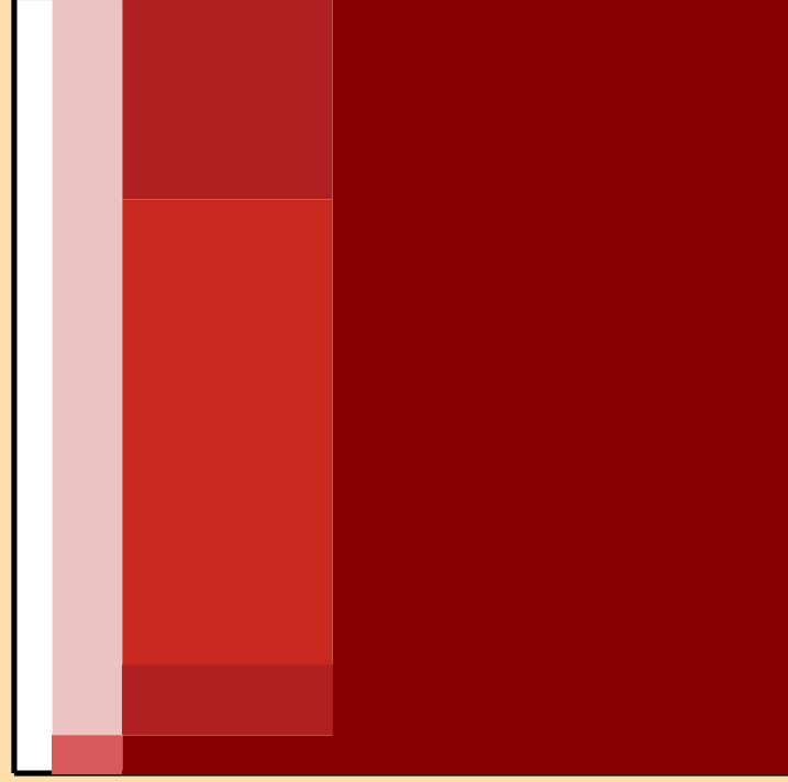
\Delta\sigma/\sigma vs. E for ^{260}\text{Fm}(n,2n)
