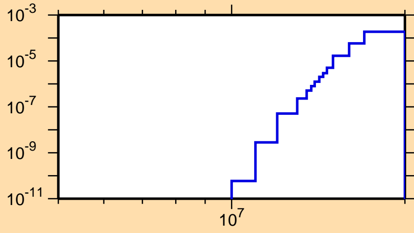
\sigma vs. E for ^{260}\text{Fm}(n,d)
