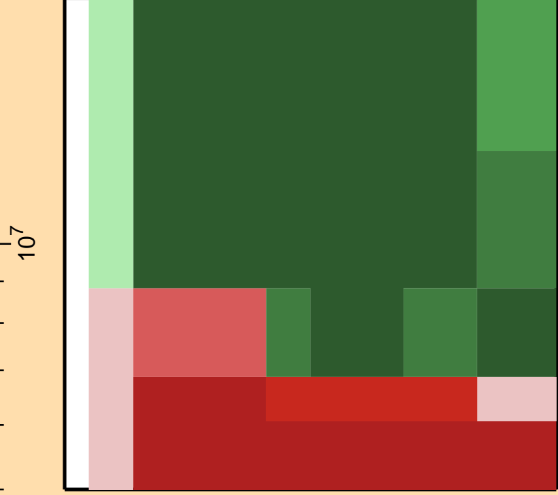
\Delta\sigma/\sigma vs. E for ^{260}\text{Fm}(n,2n)
