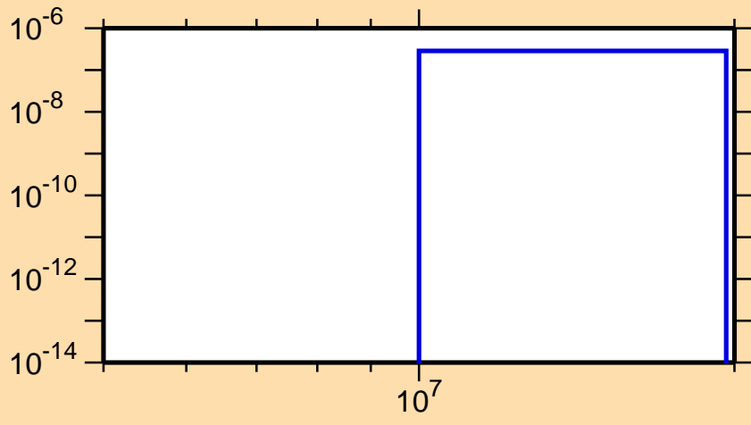
\sigma vs. E for ^{260}\text{Fm}(n,np)
