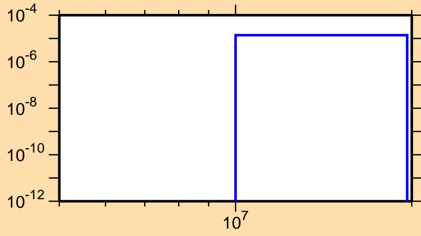
\sigma vs. E for ^{260}\text{Fm}(n,t)
