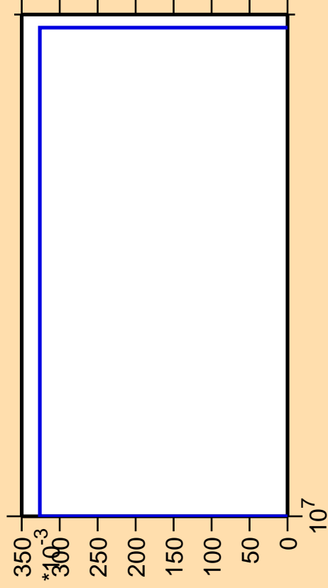
\Delta\sigma/\sigma vs. E for ^{260}\text{Fm}(n,3n\alpha)
