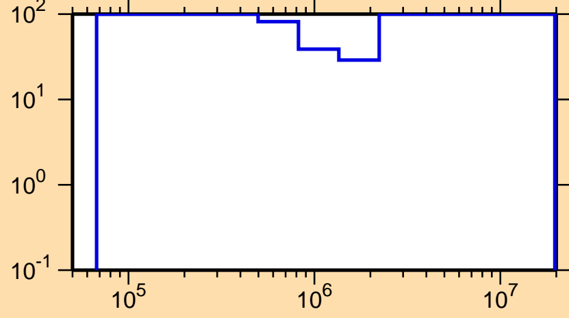
\Delta\sigma/\sigma vs. E for ^{260}\text{Fm}(n,ncont.)
