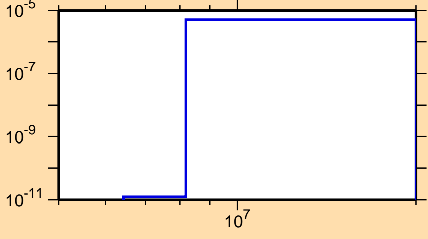
\sigma vs. E for ^{260}\text{Fm}(n,\alpha)
