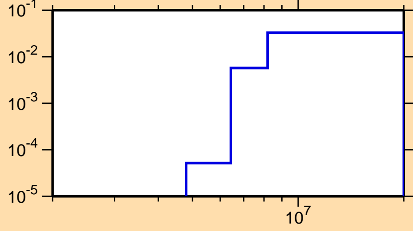
\sigma vs. E for ^{260}\text{Fm}(n,2n)
