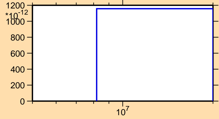
\sigma vs. E for ^{260}\text{Fm}(n,2n\alpha)
