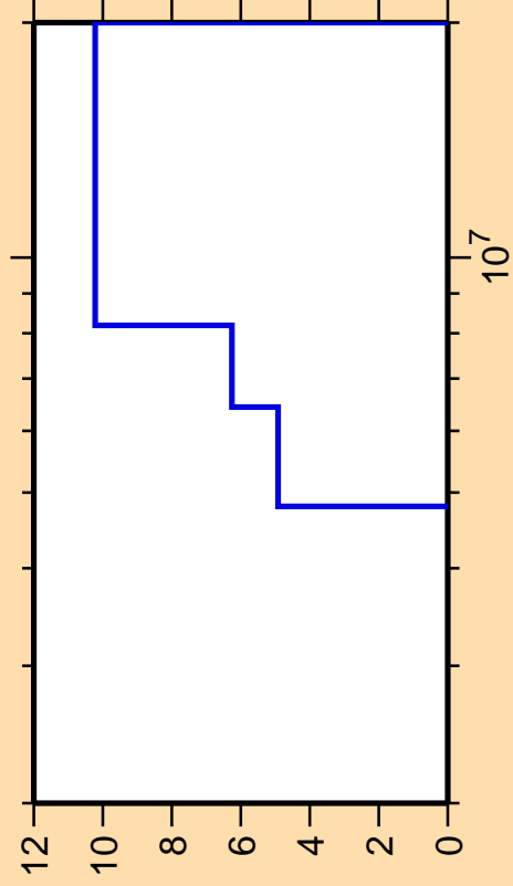
\Delta\sigma/\sigma vs. E for ^{260}\text{Fm}(n,f)
