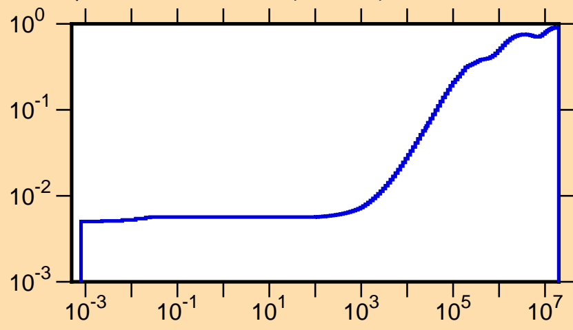
\mu vs. E for ^{135}\text{Gd}(\text{mt251})
