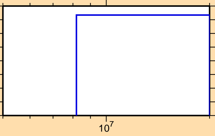
\sigma vs. E for ^{135}\text{Gd}(n,\text{pt})
