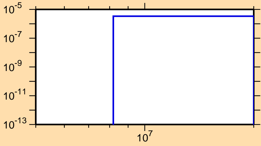
\sigma vs. E for ^{135}\text{Gd}(\text{mt } 45)
