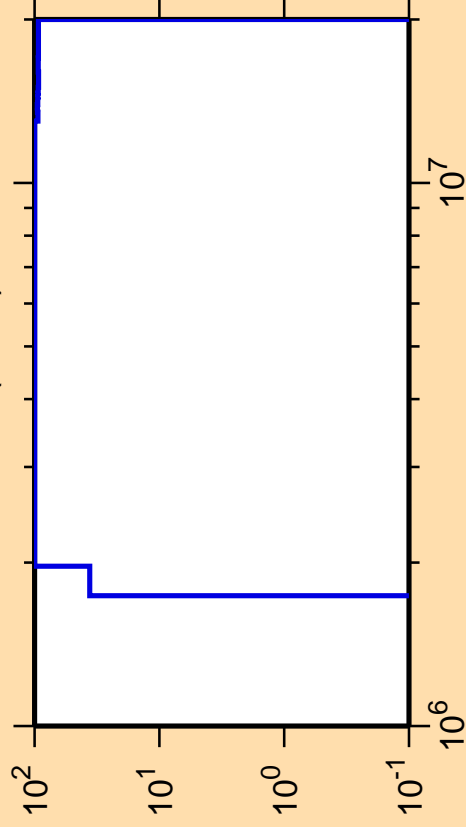
\Delta\sigma/\sigma vs. E for ^{136}\text{Gd}(n,n\alpha)
