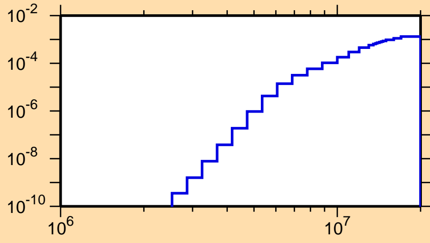
\sigma vs. E for ^{136}\text{Gd}(n,n\alpha)
