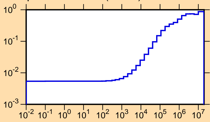
\mu vs. E for ^{136}\text{Gd}(\text{mt251})
