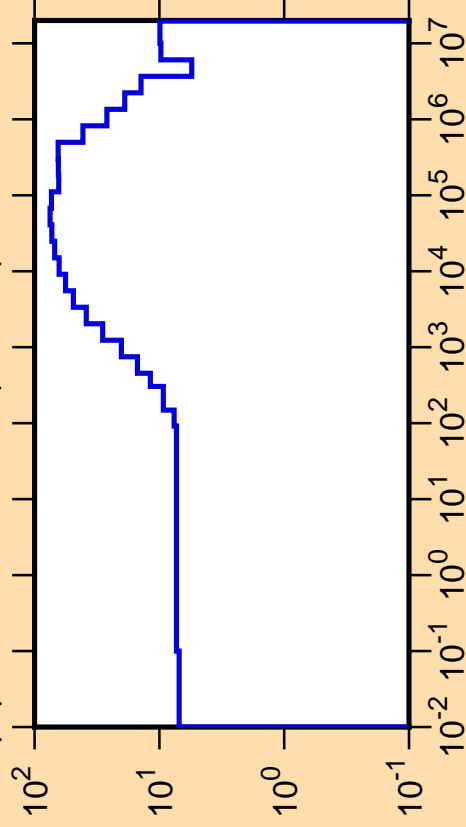
\Delta\mu/\mu vs. E for ^{136}\text{Gd}(\text{mt251})
