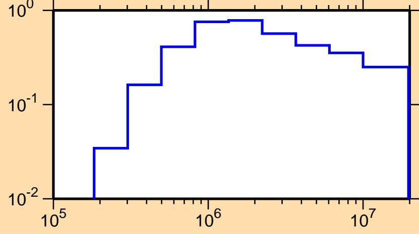
\sigma vs. E for ^{136}\text{Gd}(n,\text{inel.})
