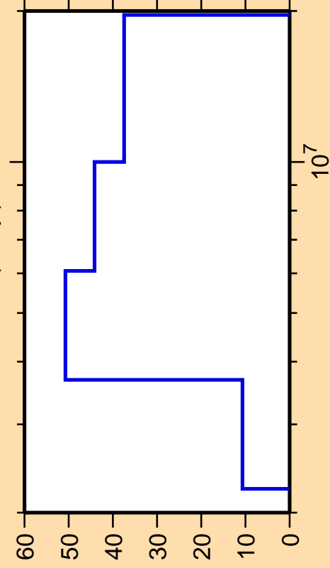
\Delta\sigma/\sigma vs. E for ^{136}\text{Gd}(n,np)
