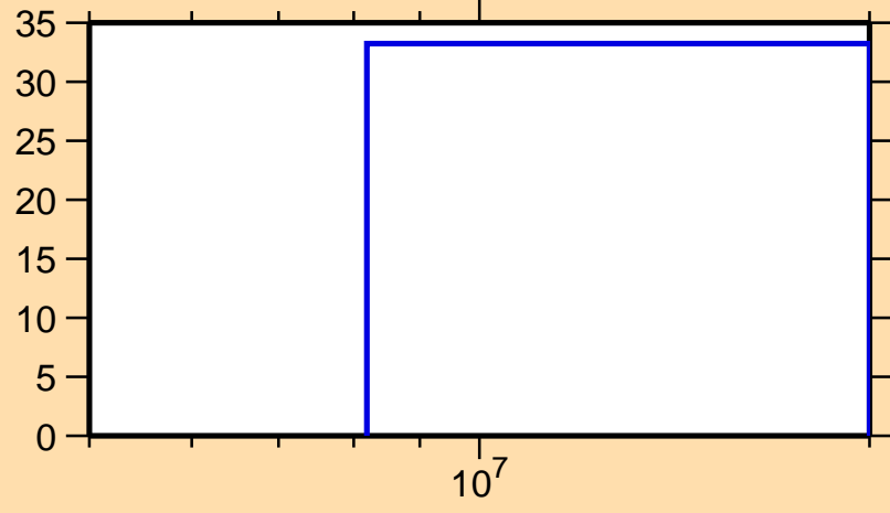
\Delta\sigma/\sigma vs. E for ^{136}\text{Gd}(n,\text{inel.})
