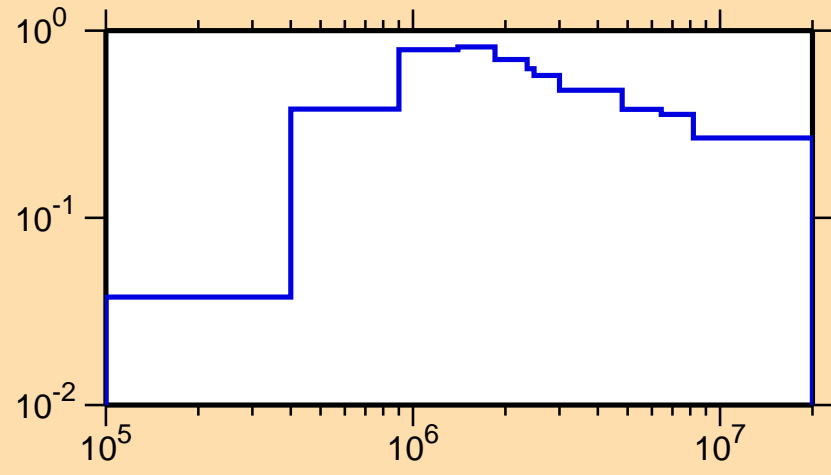
\sigma vs. E for ^{136}\text{Gd}(n,\text{inel.})
