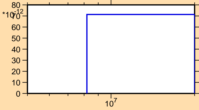
\sigma vs. E for ^{136}\text{Gd}(n,nd)
