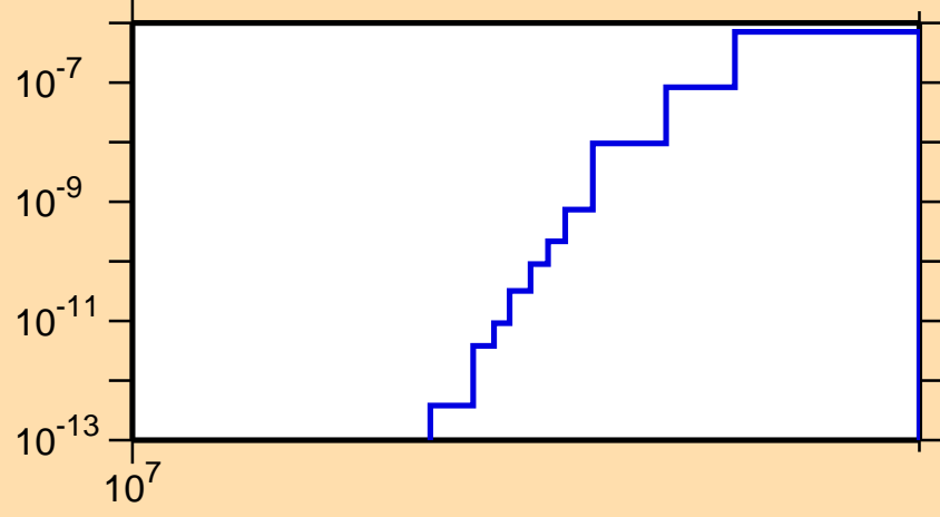
\sigma vs. E for ^{137}\text{Gd}(n,nd)
