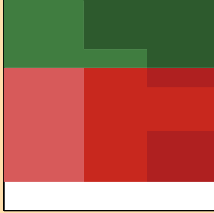
\Delta\sigma/\sigma vs. E for ^{137}\text{Gd}(n,\text{inel.})
