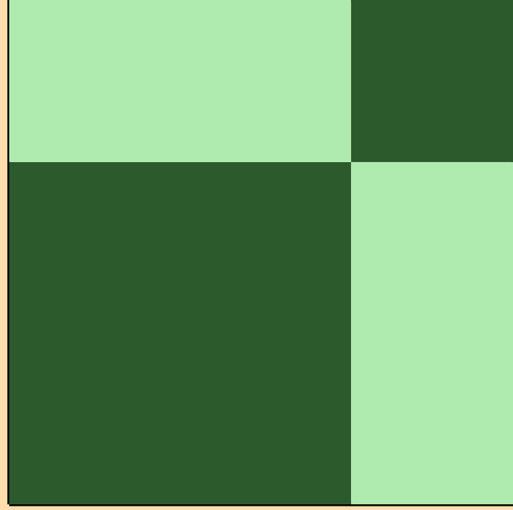
\sigma vs. E for ^{137}\text{Gd}(n,2n)
