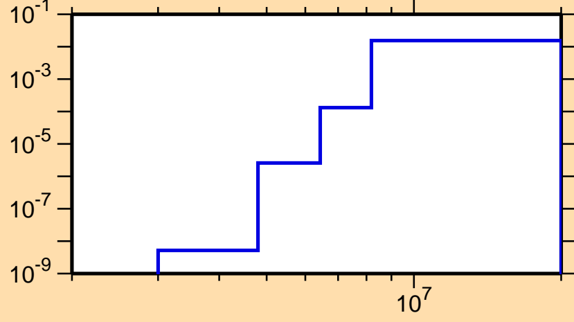
\sigma vs. E for ^{137}\text{Gd}(n,d)
