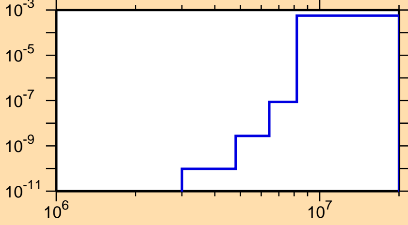
\sigma vs. E for ^{137}\text{Gd}(n,\text{He3})
