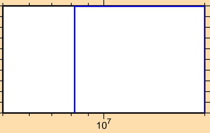
\sigma vs. E for ^{137}\text{Gd}(\text{mt117})
