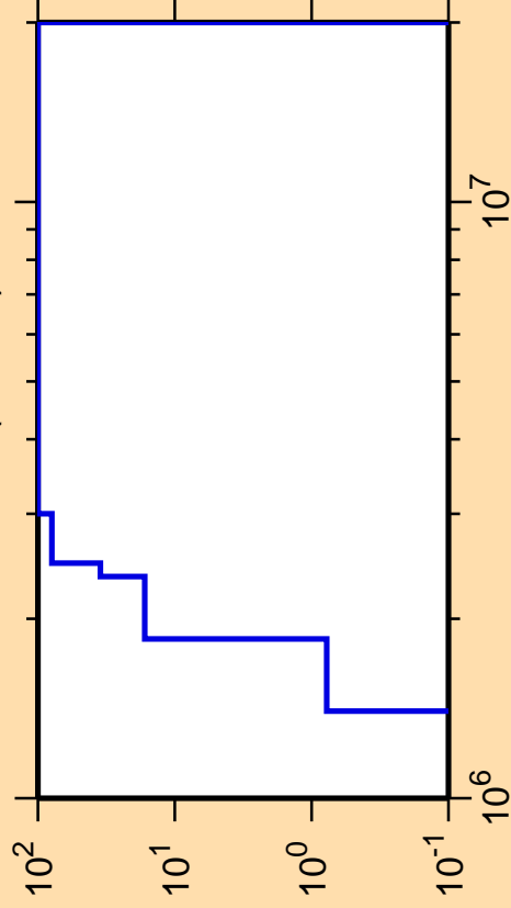
\Delta\sigma/\sigma vs. E for ^{137}\text{Gd}(n,\text{He3})
