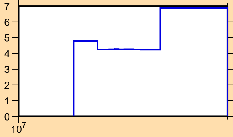
\Delta\sigma/\sigma vs. E for ^{138}\text{Gd}(n,\text{tot.})
