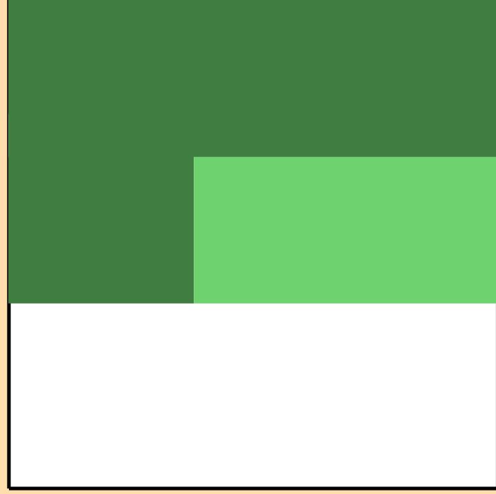
\Delta\sigma/\sigma vs. E for ^{138}\text{Gd}(n,\text{inel.})
