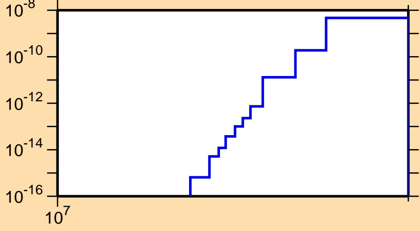
\sigma vs. E for ^{138}\text{Gd} (mt 34)
