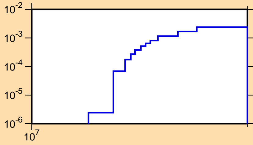
\sigma vs. E for ^{138}\text{Gd}(n,2n)
