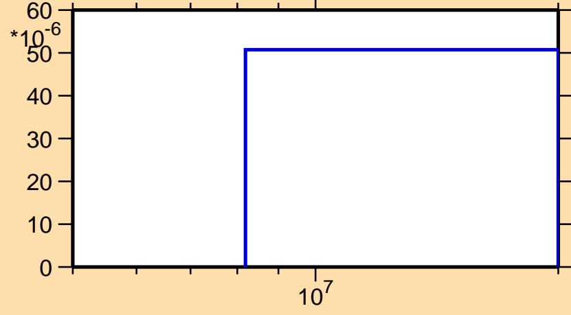
\sigma vs. E for ^{138}\text{Gd}(n,t)
