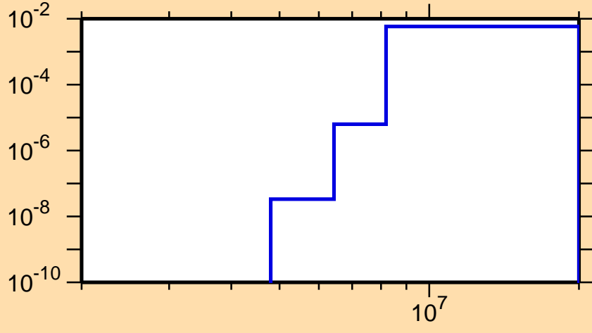
\sigma vs. E for ^{138}\text{Gd}(n,d)
