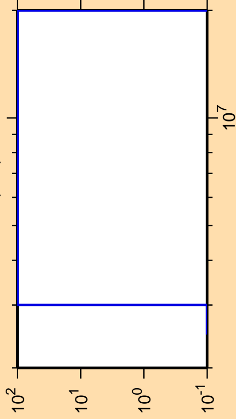
\Delta\sigma/\sigma vs. E for ^{138}\text{Gd}(n,d)
