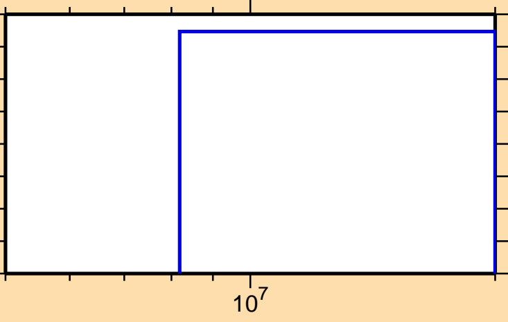
\sigma vs. E for ^{138}\text{Gd}(\text{mt117})
