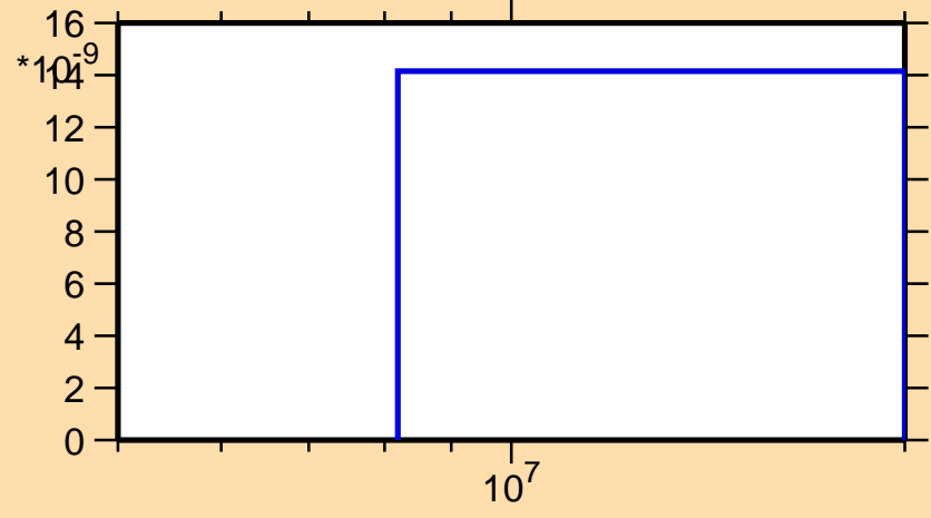
\sigma vs. E for ^{138}\text{Gd}(n,2np)
