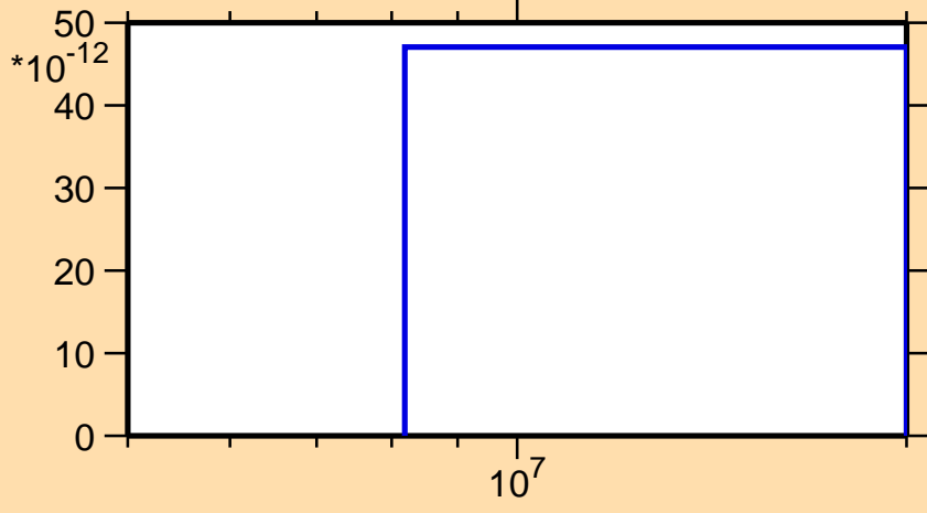
\sigma vs. E for ^{138}\text{Gd}(\text{mt } 34)
