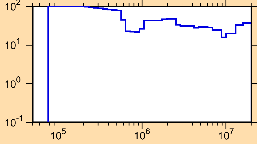
\Delta\sigma/\sigma vs. E for ^{139}\text{Gd}(n,\text{el.})
