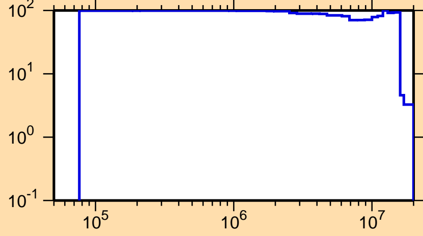
\Delta\sigma/\sigma vs. E for ^{139}\text{Gd}(n,n_1)
