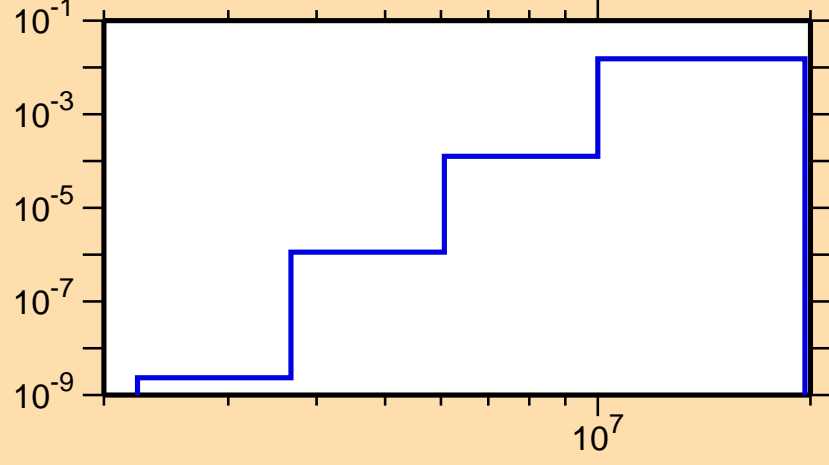
\sigma vs. E for ^{139}\text{Gd}(n,n\alpha)
