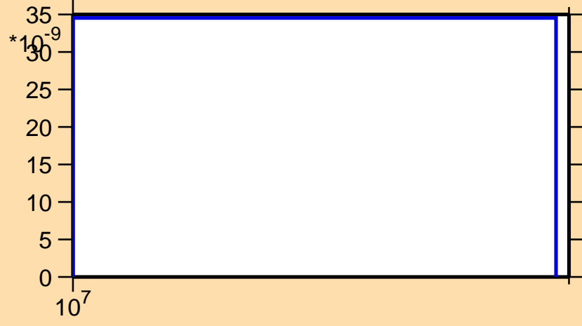
\sigma vs. E for ^{139}\text{Gd}(n,\text{nd})
