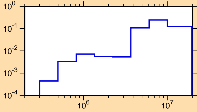
\sigma vs. E for ^{139}\text{Gd}(n,n\text{cont.})
