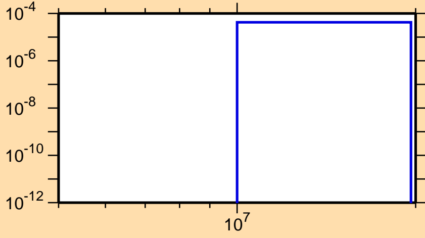
\sigma vs. E for ^{139}\text{Gd}(n,\text{pt})
