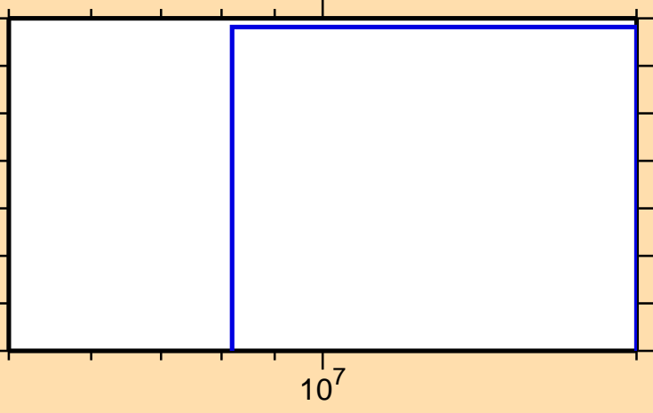
\sigma vs. E for ^{139}\text{Gd}(n,\text{pt})
