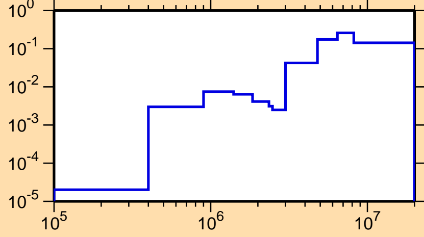
\sigma vs. E for ^{139}\text{Gd}(n,n\text{cont.})
