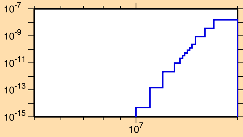
\sigma vs. E for ^{140}\text{Gd}(\text{mt117})
