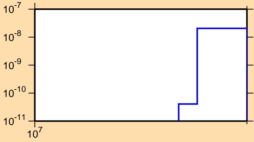
\sigma vs. E for ^{140}\text{Gd}(n,\text{nd})
