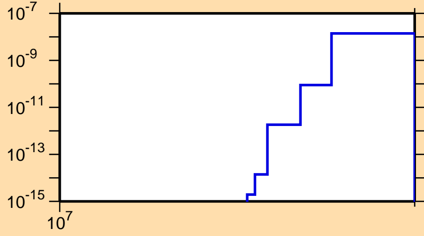
\sigma vs. E for ^{140}\text{Gd}(n,2n\alpha)
