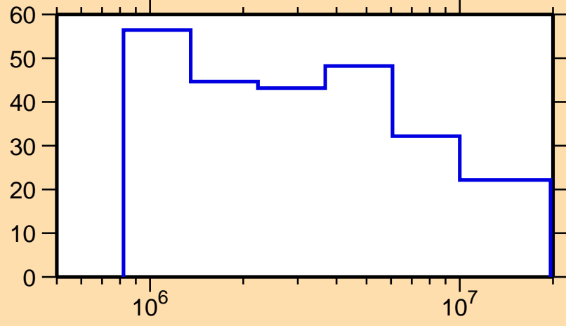
\Delta\sigma/\sigma vs. E for ^{140}\text{Gd}(n,\text{inel.})
