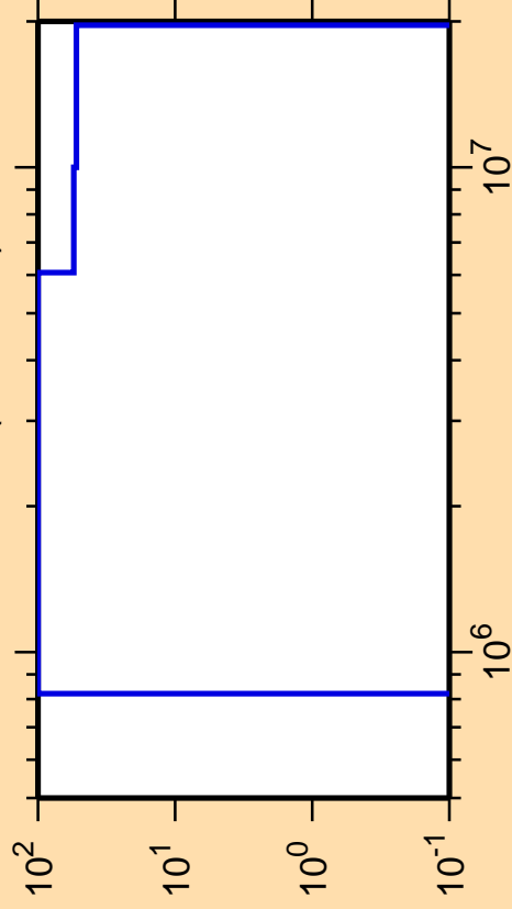
\Delta\sigma/\sigma vs. E for ^{140}\text{Gd}(n,n\text{cont.})
