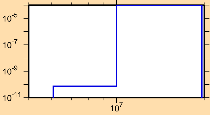
\sigma vs. E for ^{140}\text{Gd}(n,\text{pd})
