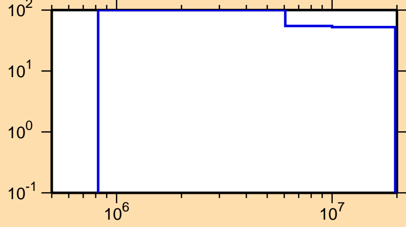
\Delta\sigma/\sigma vs. E for ^{140}\text{Gd}(n,n\text{cont.})
