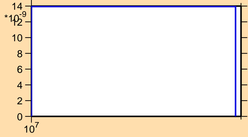
\sigma vs. E for ^{140}\text{Gd}(n,2np)
