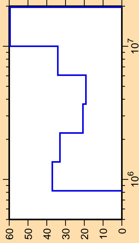
\Delta\sigma/\sigma vs. E for ^{140}\text{Gd}(n,p)
