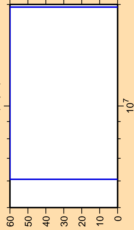
\Delta\sigma/\sigma vs. E for ^{140}\text{Gd}(n,\text{pd})
