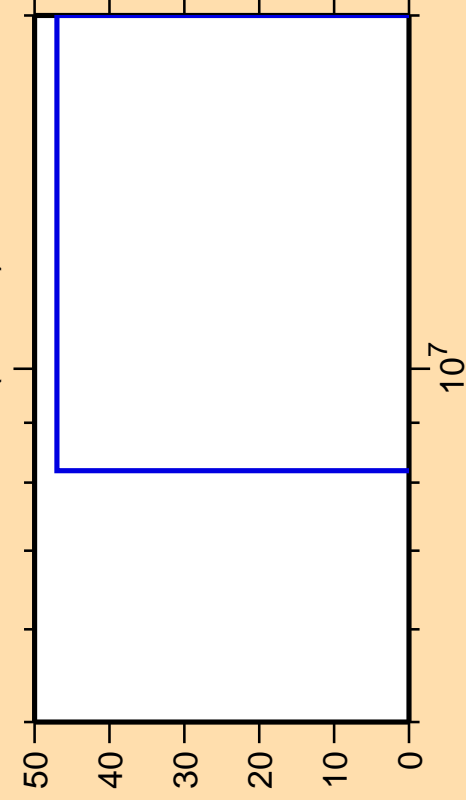
\Delta\sigma/\sigma vs. E for ^{140}\text{Gd}(\text{mt } 34)
