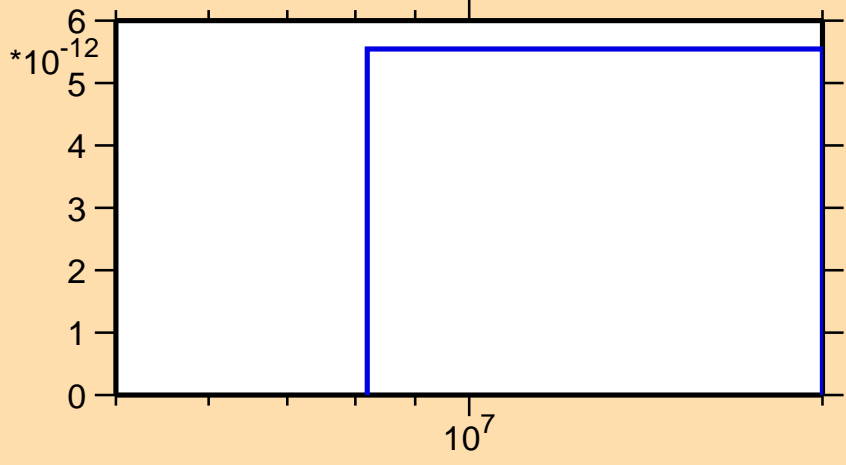
\sigma vs. E for ^{140}\text{Gd}(\text{mt } 34)
