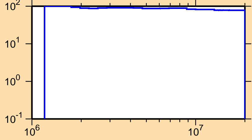
\Delta\sigma/\sigma vs. E for ^{141}\text{Gd}(n,n\text{cont.})
