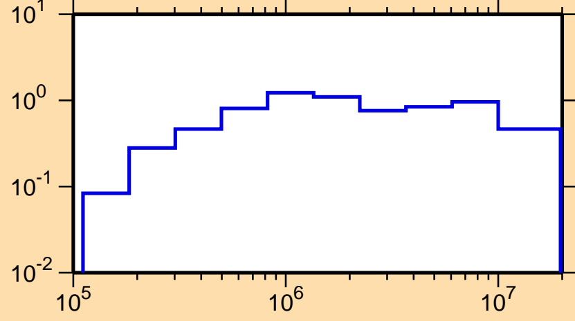
\sigma vs. E for ^{141}\text{Gd}(n,\text{inel.})
